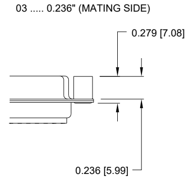
#4-40 INTERNAL THREADS
