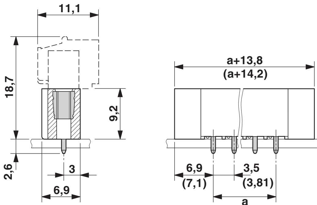
Dimensional drawing
