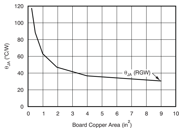
Figure 44. \theta_{JA} vs Board Size
