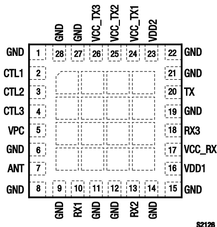
Figure 1. SKY65313-21 Pinout (Top View)
