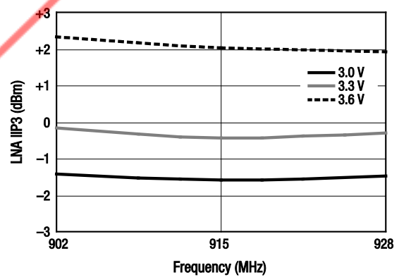
Figure 16. LNA IIP3 vs Frequency Over VCC_RX (VCC_TX/1/2/3 = VDD2 = 4.0 V, Tc = 25 °C)
