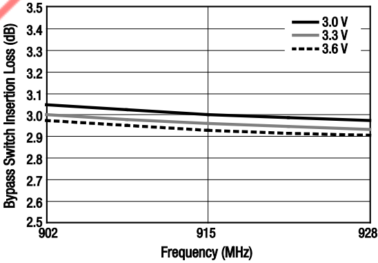
Figure 22. Bypass Switch Insertion Loss vs Frequency Over VCC_RX (VCC_TX/1/2/3 = VDD2 = 4.0 V, Tc = 25 °C)
