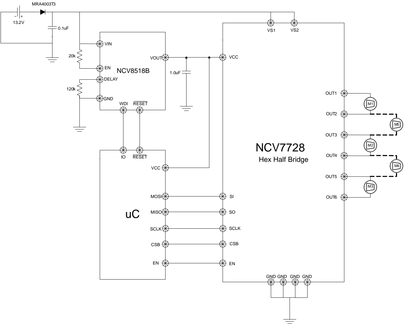
Figure 29. Application Drawing
