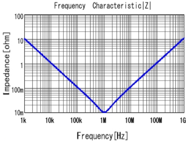
■ ECASD41E156M040KA0 |Z| DC0V, 25degC
