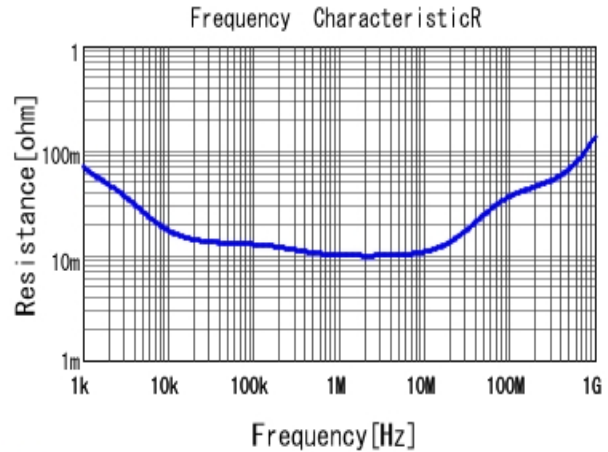
■ ECASD41E156M040KA0 R DC0V, 25degC
