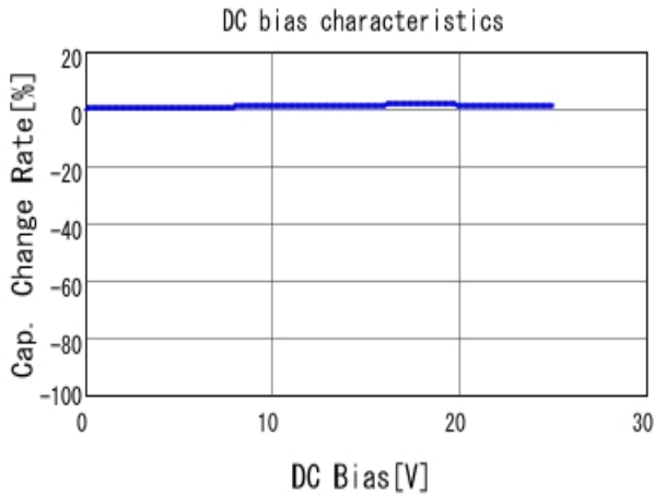
■ ECASD41E156M040KA0 C-DC bias capchange, 25.0degC, AC1
