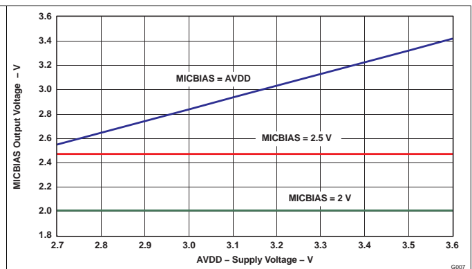
Figure 35. MICBIAS Output Voltage vs AVDD
