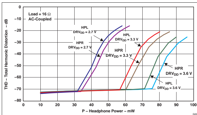
Figure 34. Headphone Power vs THD, 16- \Omega Load
