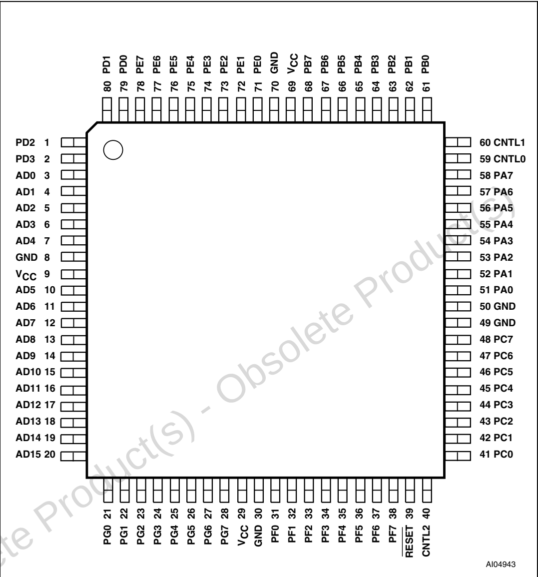
Figure 1. LQFP80 connections
