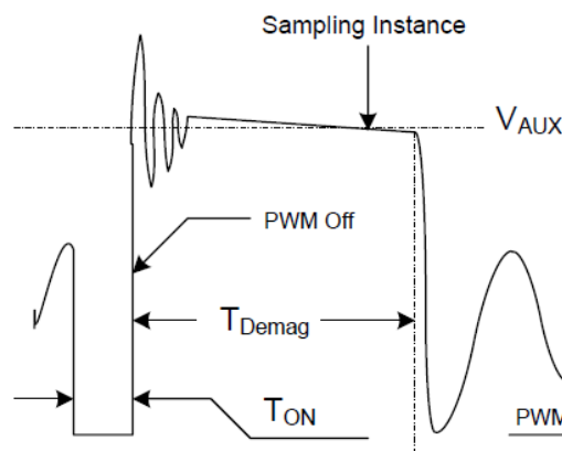
Fig.2. Auxiliary voltage waveform
