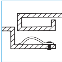
RIVET MOUNT
