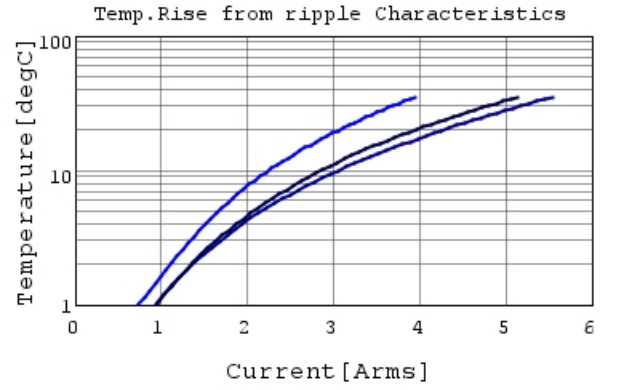
GRM31CR71A475KA01 Temp.rise — 100kHz —
