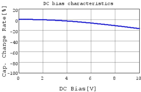
GRM31CR71A475KA01 C-DC bias capchange, 25.0c
