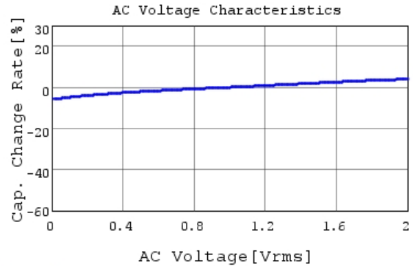
GRM31CR71A475KA01 C-AC Voltage capchange, DC
