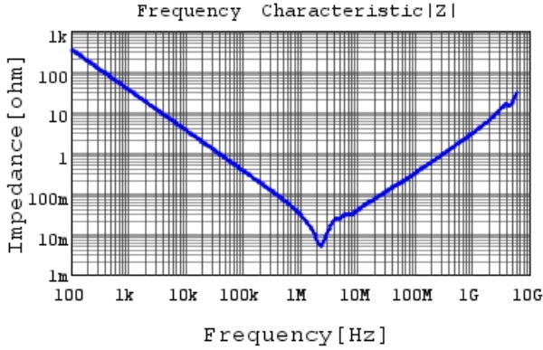
GRM31CR71A475KA01 |Z| DCOV, 25degC
