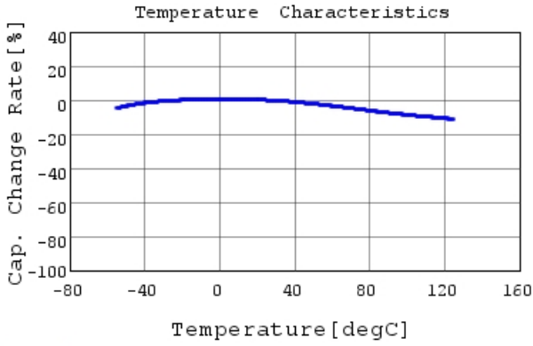
GRM31CR71A475KA01 C-Temp. capchange, DC0.0V,
