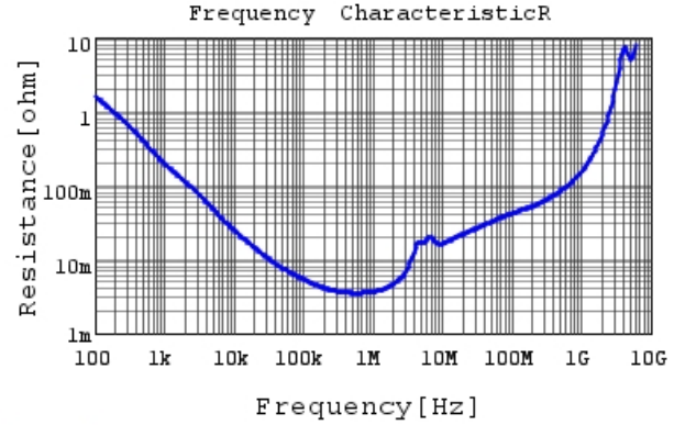
GRM31CR71A475KA01 R DCOV, 25degC
