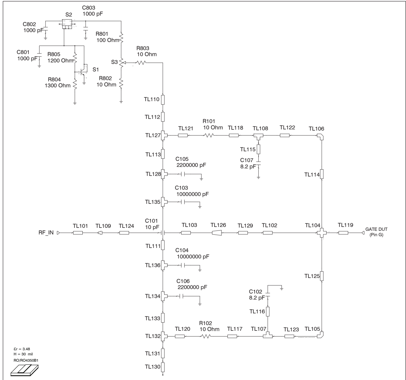
Reference circuit input schematic for f = 1990 \text{ MHz}
