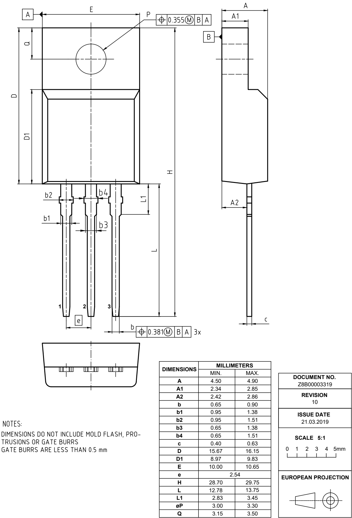
Figure 1 Outline PG-TO220 FullPAK, dimensions in mm
