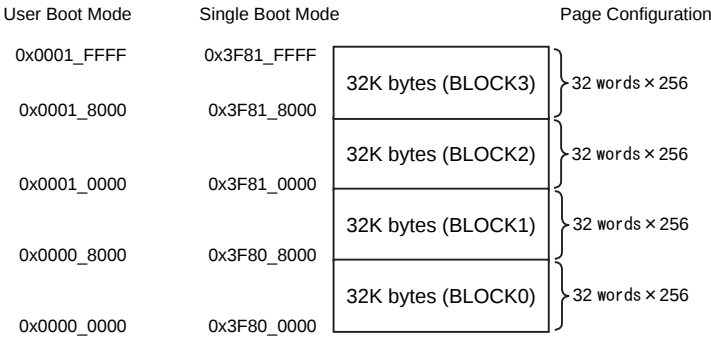
Figure 17-1 Block configuration
