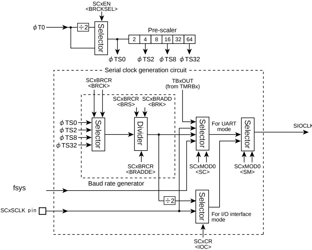
Figure 12-2 Serial clock generation circuit block diagram
