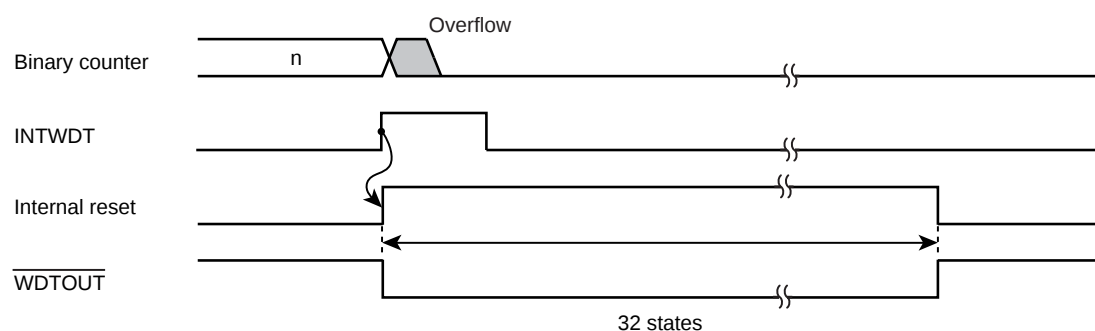
Figure 16-3 Internal reset generation
