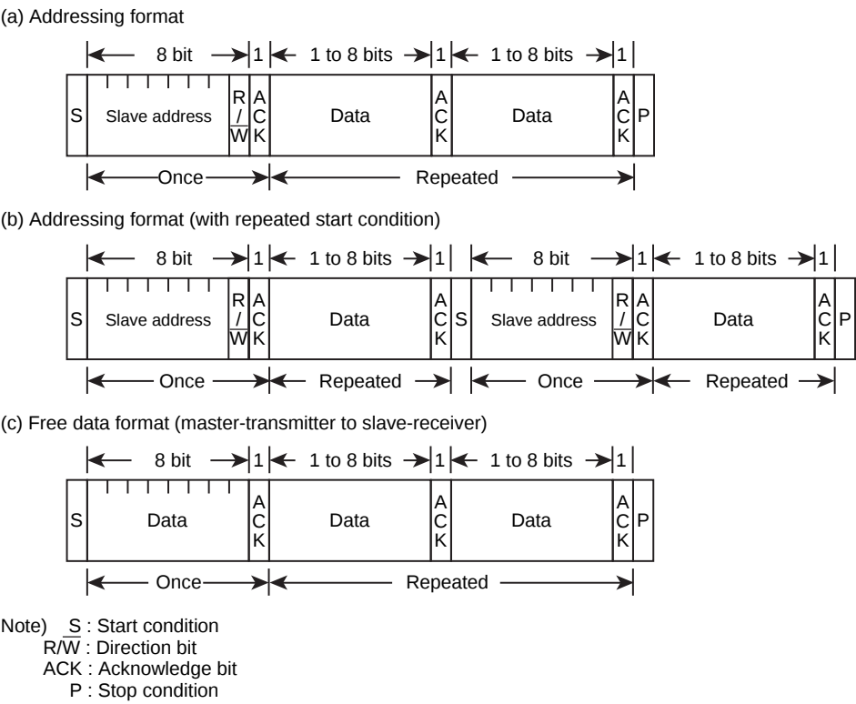
Figure 13-3 I2C Bus Mode Data Formats
