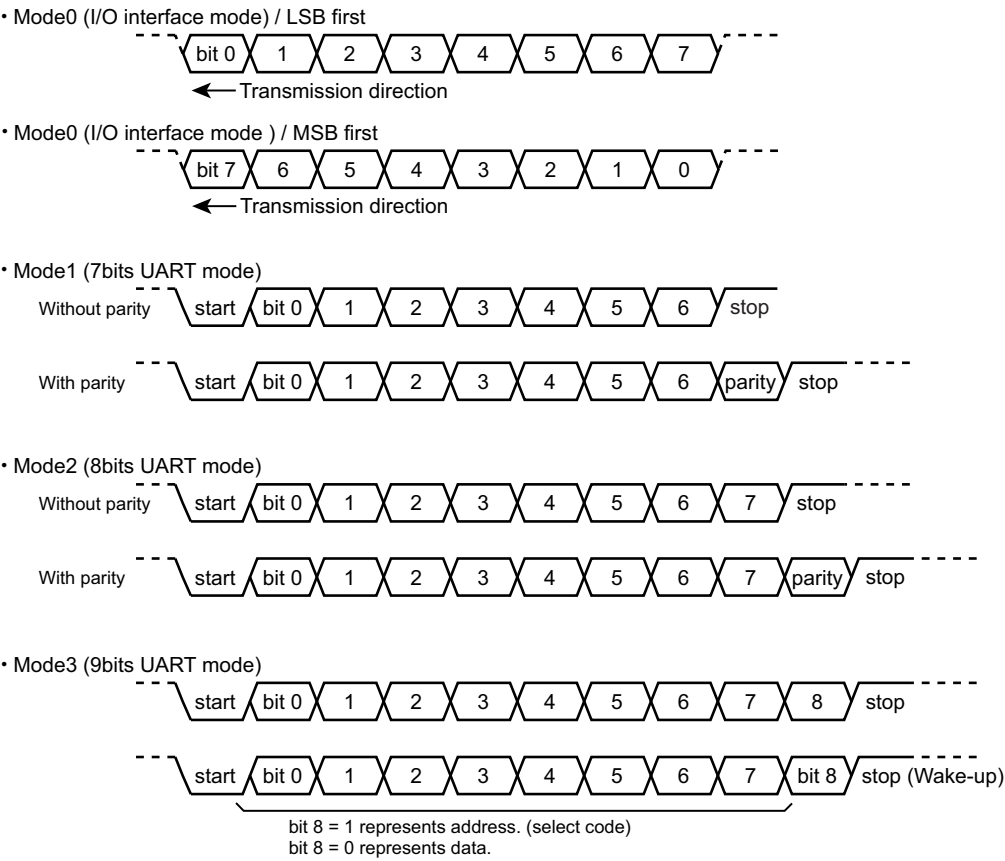
Figure 12-3 Data Format
