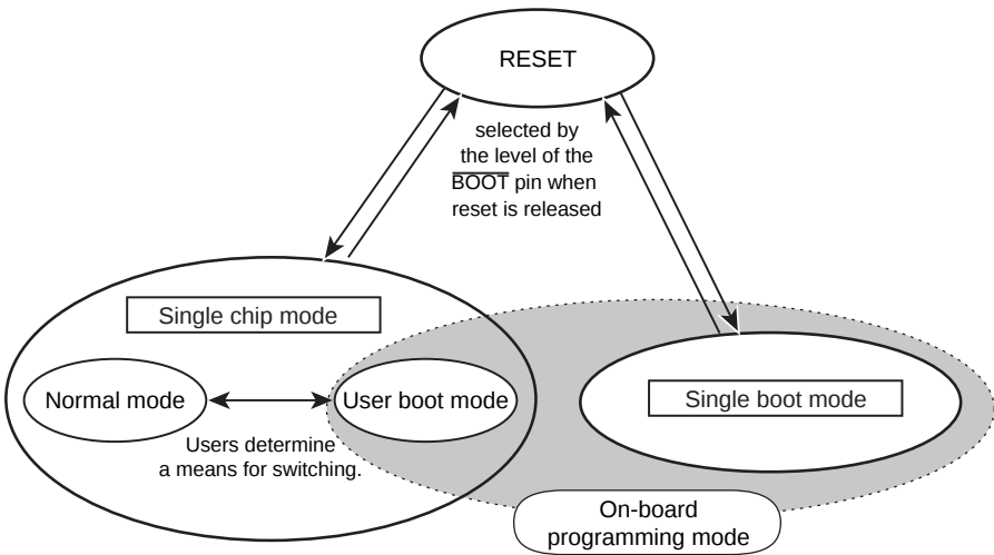
Figure 17-2 Mode transition
