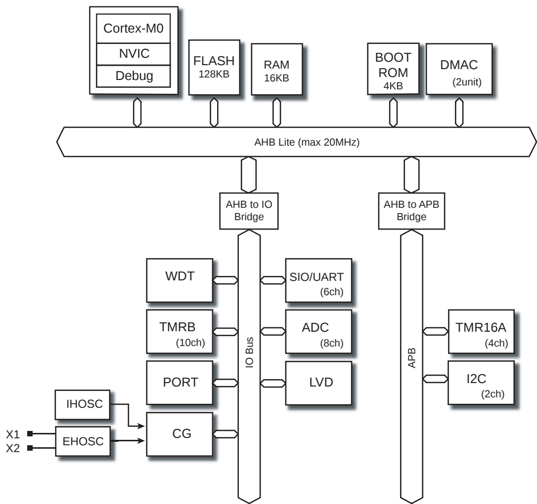
Figure 1-1 Block Diagram
