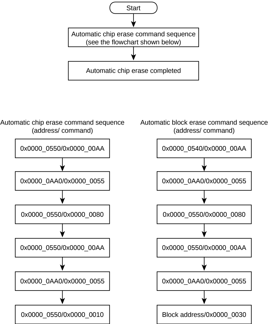
Figure 17-5 Flowchart of automatic erase
