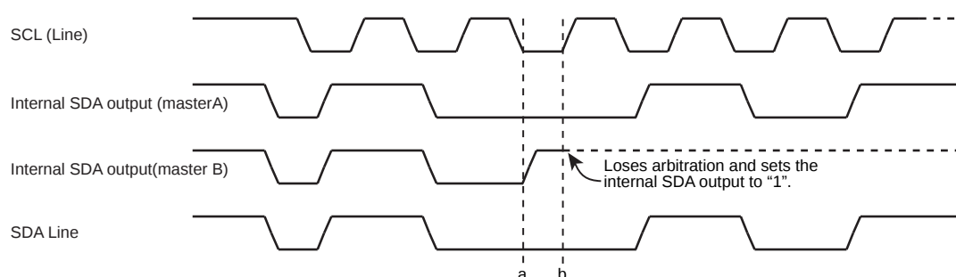
Figure 13-8 Lost Arbitration
