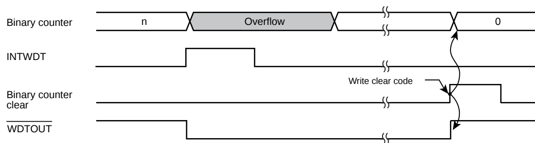
Figure 16-2 INTWDT interrupt generation
