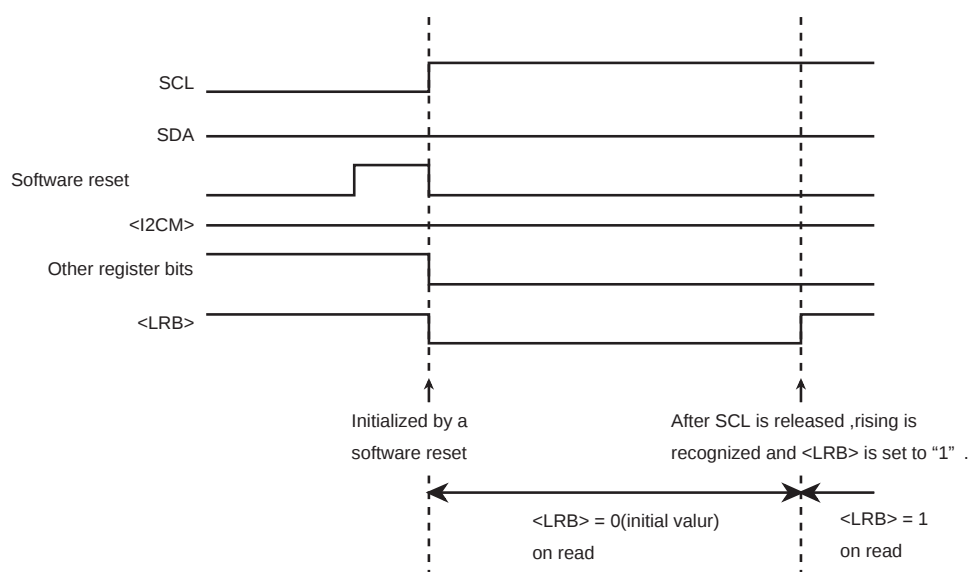
Figure 13-16 Software reset release to the SCL0 "0" to "1" while SDA="1"
