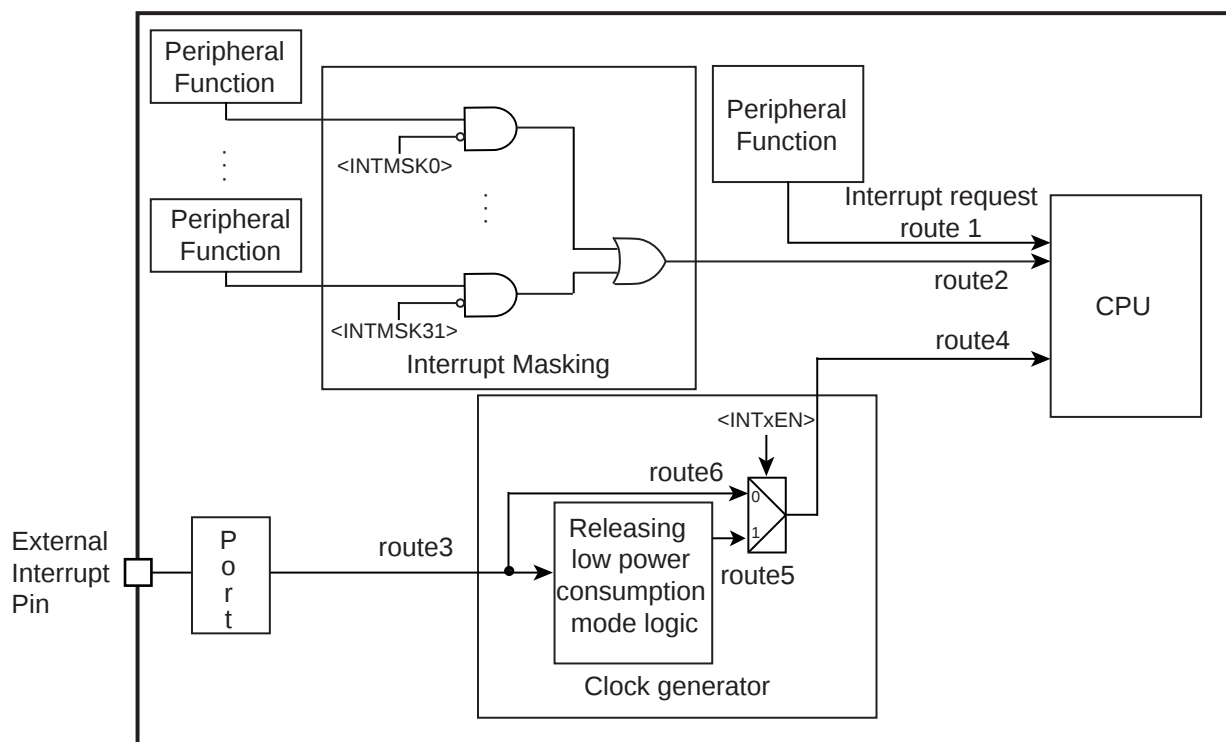
Figure 7-1 Interrupt Route
