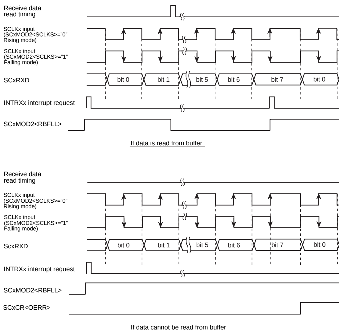
Figure 12-18 Receive Operation in the I/O Interface Mode (Clock Input Mode)
