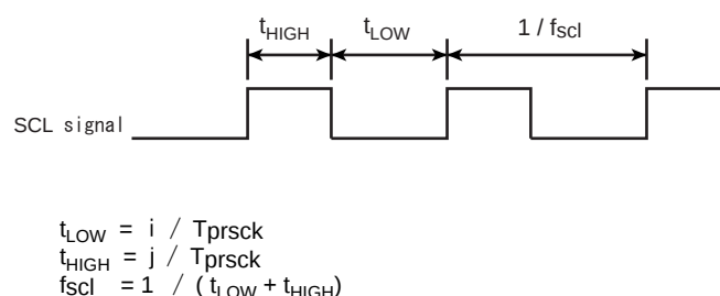
Figure 13-4 Clock source
