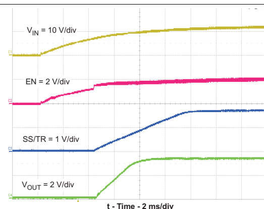
Figure 36. Start-Up With VIN (1.1-Ω Load)
