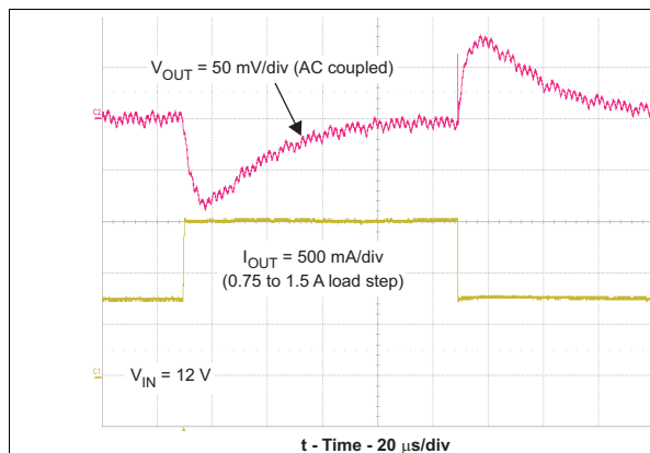
Figure 35. Load Transient
