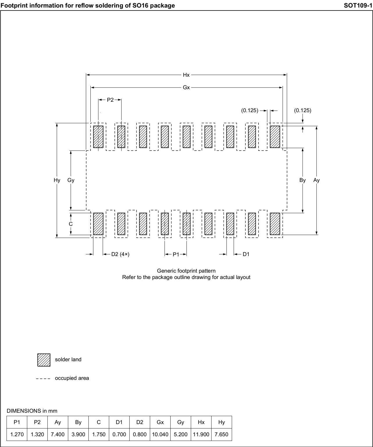
Fig 22. PCB footprint for SOT109-1 (SO16); reflow soldering
