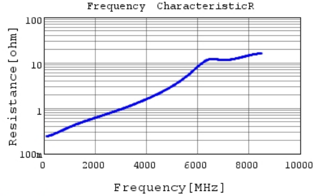
GCM1885C1H100JA16 R DCOV, 25degC
