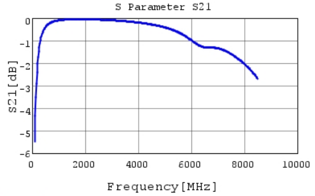
GCM1885C1H100JA16 S21 DCOV, 25degC
