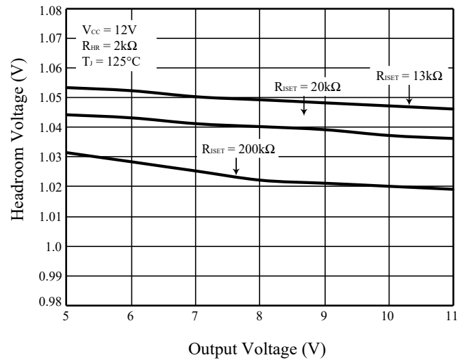
Figure 15 V_{HR} vs. V_{OUT}
