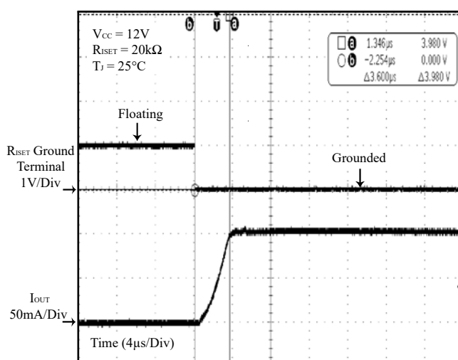
Figure 47 ISET PWM On Delay Time for IS32LT3124B/C/E/F
