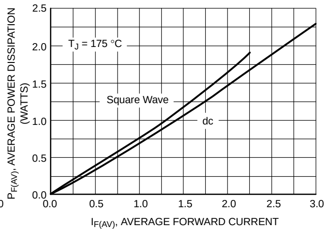
Figure 6. Power Dissipation
