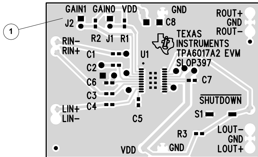
Figure 2–1. Module Preparation
