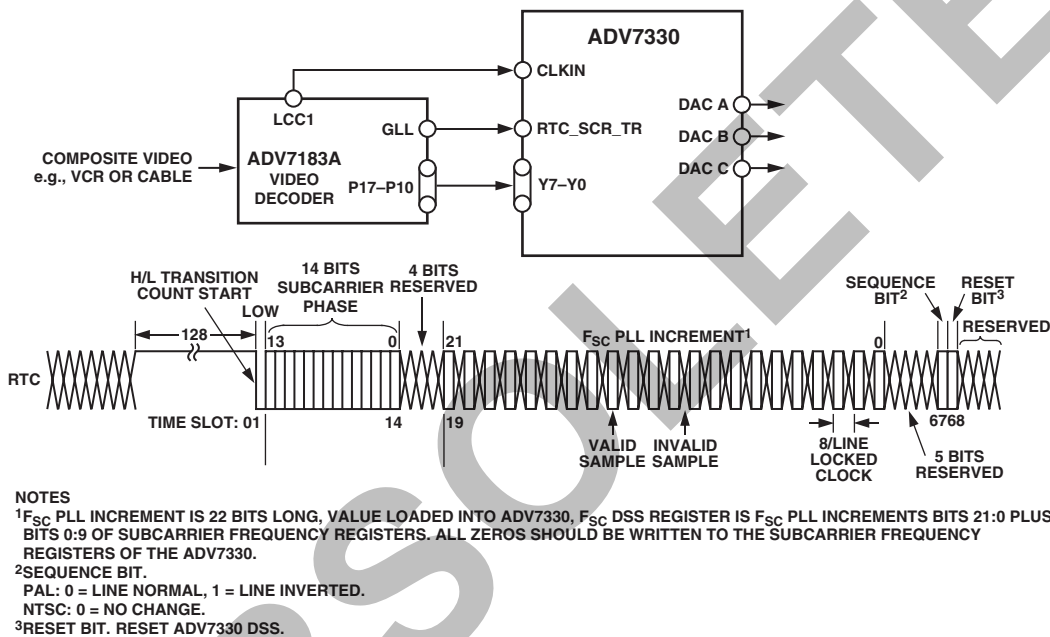
Figure 23. RTC Timing and Connections
