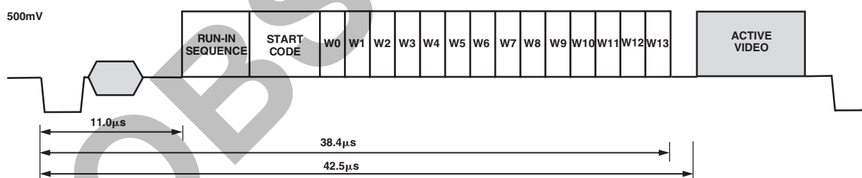
Figure 57. WSS Waveform Diagram
