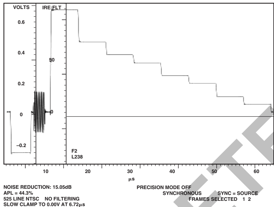
Figure 99. NTSC Luma
