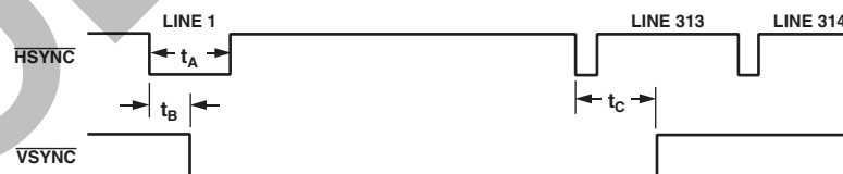
Figure 15. Timing Register 1 in PAL Mode
