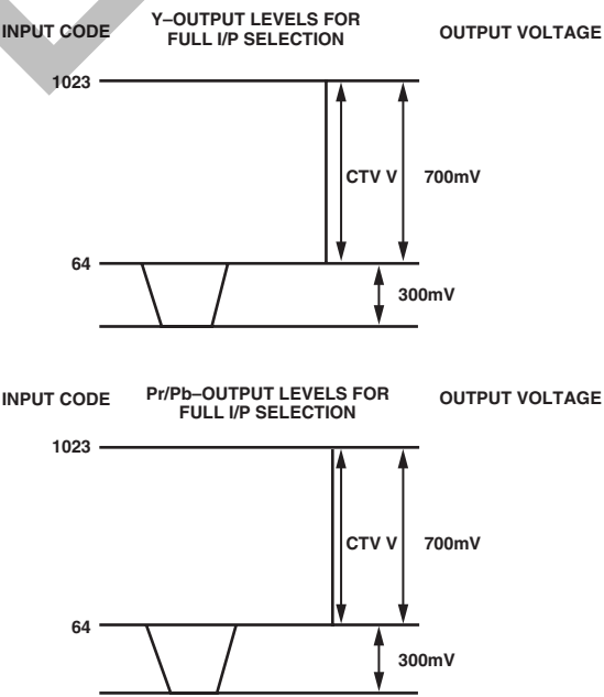
Figure 86. Output Levels for Full I/P Selection
