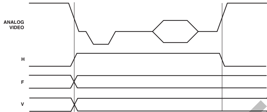
Figure 72. SD Master Mode 0, Data Transitions
