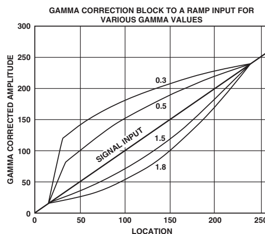
Figure 33. Signal Input (Ramp) and Selectable Gamma Output Curves
