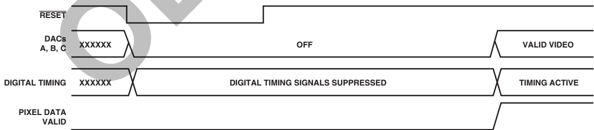
Figure 24. \overline{\text{RESET}} Timing Sequence
