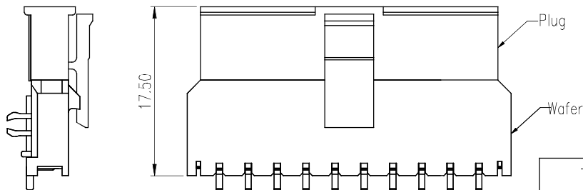
MATED MICRO POWER CONNECTOR
