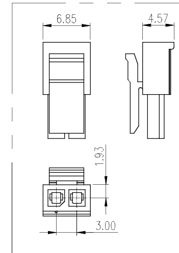
(2 CIRCUIT HOUSING)
