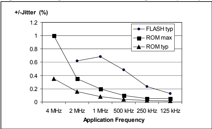
Figure 77. Integrated PLL Jitter vs signal frequency 1
