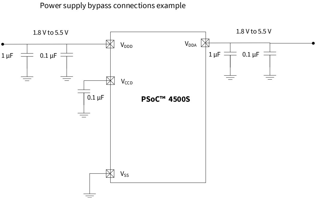
Figure 6 External supply range from 1.8 V to 5.5 V with internal regulator active
