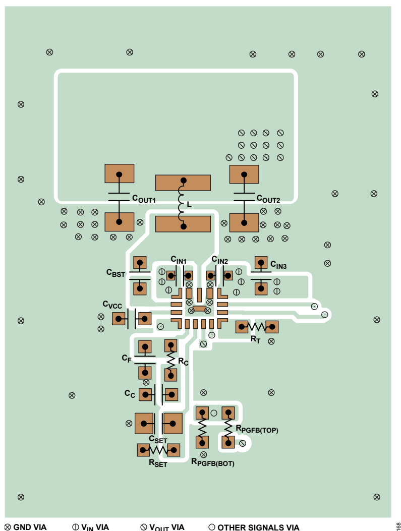
Figure 49. LT83203/LT83205 Suggested Layout
