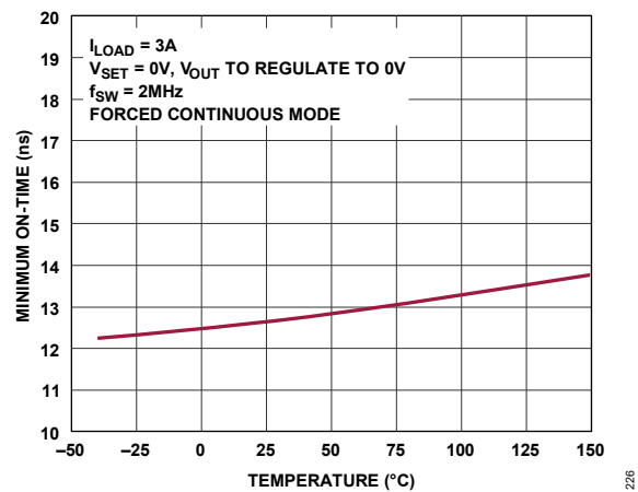
Figure 29. Minimum On-Time vs. Temperature
