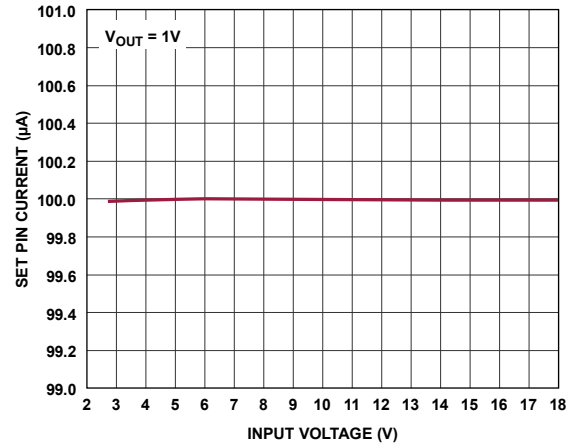
Figure 17. SET Pin Current vs. Input Voltage
