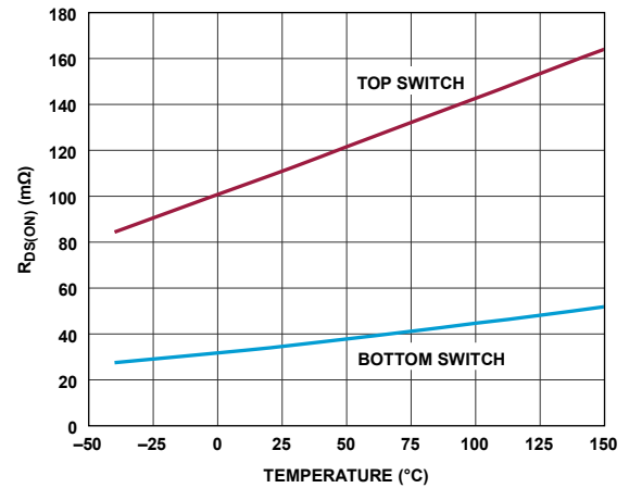
Figure 23. Switch R_{DS(ON)} vs. Temperature
