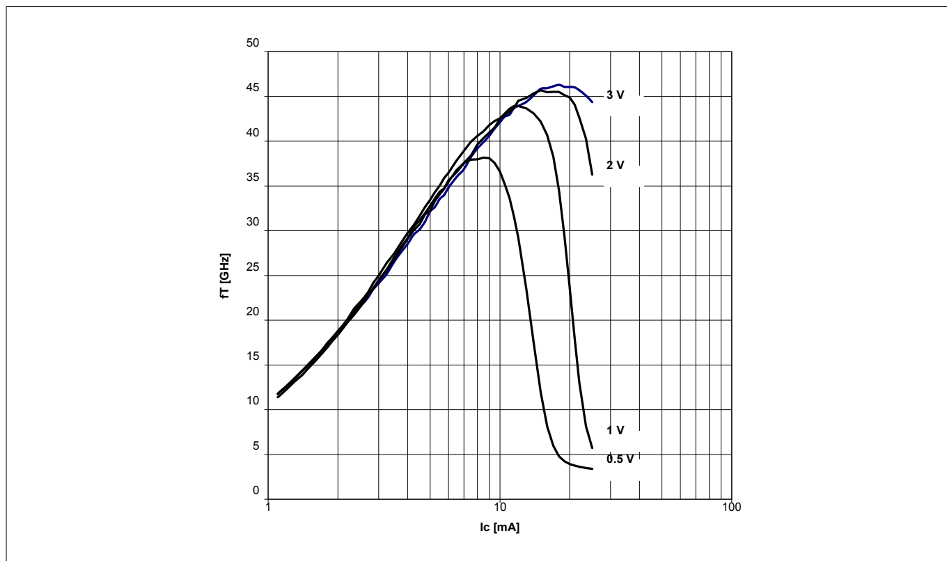
Figure 5 Transition frequency f_T = f(I_C, V_{CE}) , f = 1 GHz, V_{CE} = \text{parameter}
