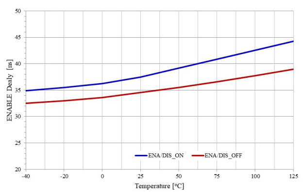
Figure 29. ENA/DIS Delay Time vs. Temperature
