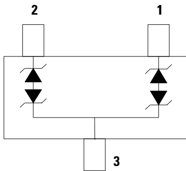
Pinout and Functional Block Diagram
