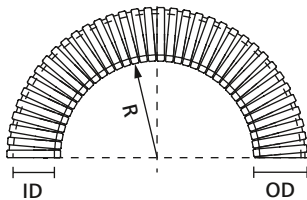
HelagaGuard non-metallic conduit
