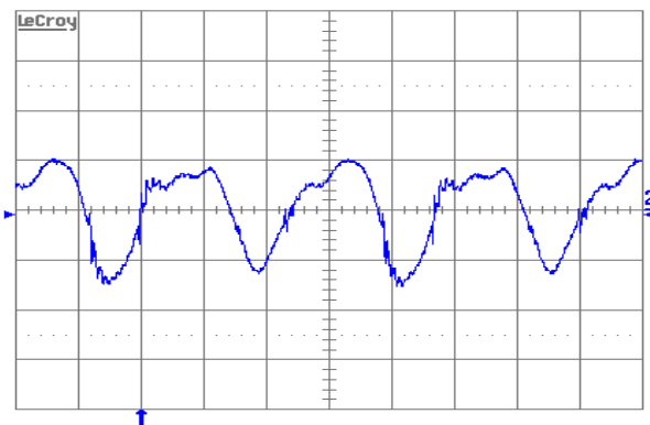
Figure 10. Output voltage ripple (20 mV/div.) at full rated load current into a resistive load with C_o = 10 \mu\text{F tantalum} + 1 \mu\text{F ceramic} and V_{in} = 48 \text{ V} . Time scale: 1 µs/div.
