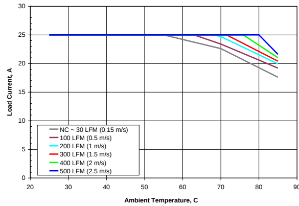
Figure 1. Available load current vs. ambient air temperature and airflow rates for SSQE48T25018 converter mounted vertically with air flowing from pin 1 to pin 3, V_{in} = 48\text{ V} . Note: NC – Natural convection
