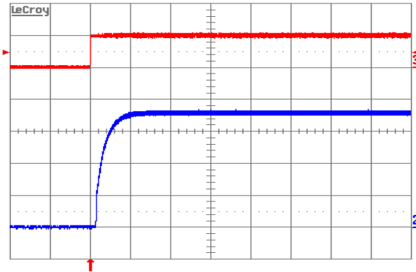
Figure 6. Turn-on transient at full rated load current (resistive) with C_o = 1 \mu\text{F cer} + 10 \mu\text{F tant} at V_{in} = 48 \text{ V} , triggered via ON/OFF pin. Top trace: ON/OFF signal (5 V/div.). Bottom trace: Output voltage (0.5 V/div.). Time scale: 5 ms/div.
