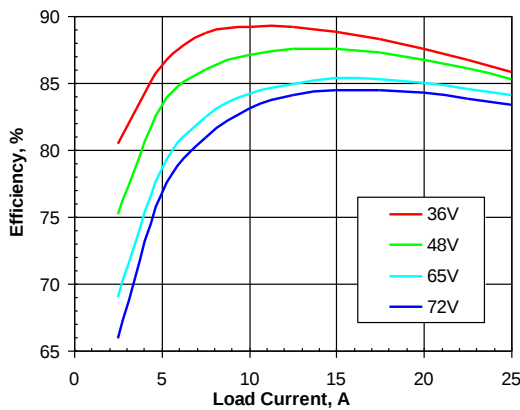
Figure 2. Efficiency vs. load current and input voltage for SSQE48T25018 converter mounted vertically with air flowing from pin 1 to pin 3 at a rate of 300 LFM (1.5 m/s) and T_a = 25^\circ\text{C} .
