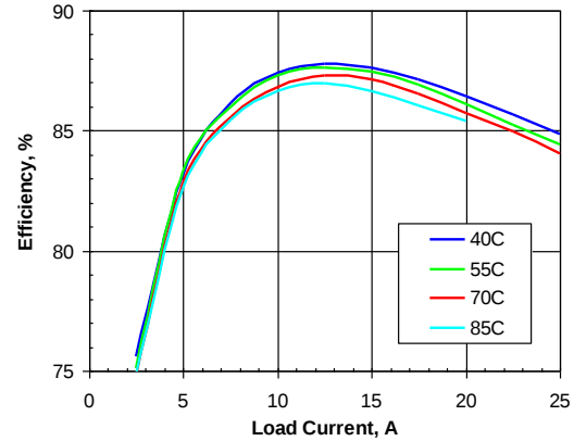
Figure 3. Efficiency vs. load current and ambient temperature for SSQE48T25018 converter mounted vertically with V_{in} = 48\text{ V} and air flowing from pin 1 to pin 3 at a rate of 200 LFM (1.0 m/s).
