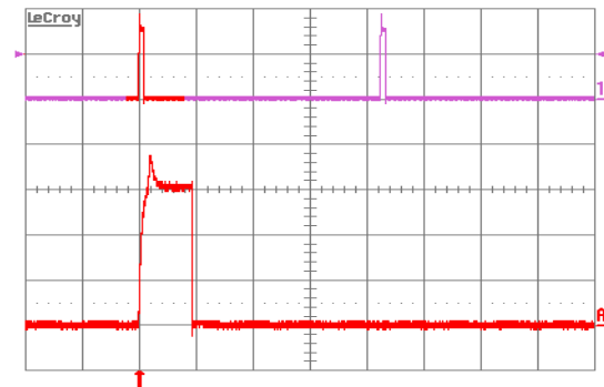
Figure 15. Load current (top trace, 20 A/div., 50 ms/div.) into a 10 m\Omega short circuit during restart, at V_{in} = 48 V. Bottom trace (10 A/div., 5 ms/div.) is an expansion of the on-time portion of the top trace.
