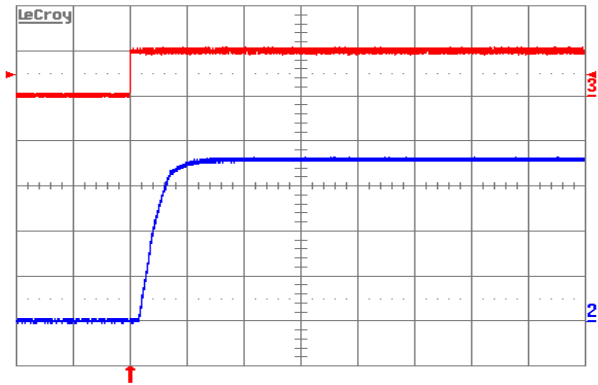
Figure 7. Turn-on transient at full rated load current (resistive) plus 30,000 \mu\text{F} at V_{in} = 48 \text{ V} , triggered via ON/OFF pin. Top trace: ON/OFF signal (5 V/div.). Bottom trace: Output voltage (0.5 V/div.). Time scale: 5 ms/div.
