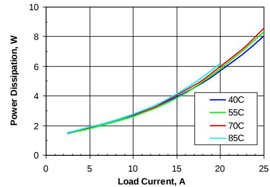
Figure 5. Power dissipation vs. load current and ambient temperature for SSQE48T25018 converter mounted vertically with V_{in} = 48\text{ V} and air flowing from pin 1 to pin 3 at a rate of 200 LFM (1.0 m/s).
