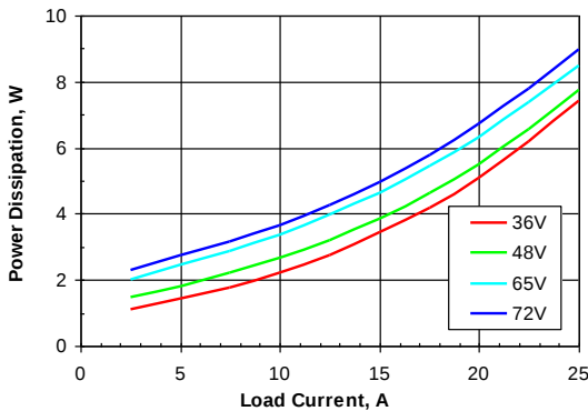
Figure 4. Power dissipation vs. load current and input voltage for SSQE48T25018 converter mounted vertically with air flowing from pin 1 to pin 3 at a rate of 300 LFM (1.5 m/s) and T_a = 25^\circ\text{C} .
