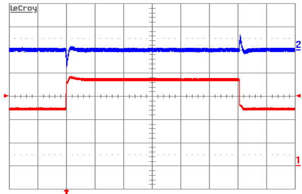
Figure 9. Output voltage response to load current step-change (12.5 A–18.75 A–12.5 A) at V_{in} = 48 \text{ V} . Top trace: output voltage (200 mV/div.). Bottom trace: load current (5 A/div.). Current slew rate: 5 A/µs. C_o = 470 \mu\text{F POS} + 1 \mu\text{F cer} . Time scale: 0.2 ms/div.
