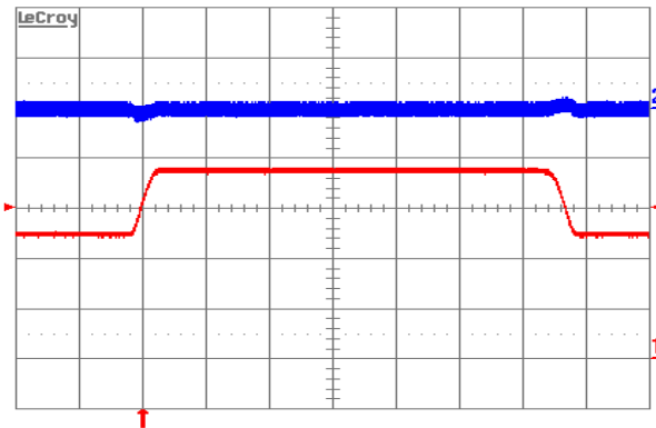
Figure 8. Output voltage response to load current step-change (12.5 A–18.75 A–12.5 A) at V_{in} = 48 \text{ V} . Top trace: output voltage (200 mV/div.). Bottom trace: load current (5 A/div.). Current slew rate: 0.1 A/µs. C_o = 1 \mu\text{F cer} + 10 \mu\text{F tant} . Time scale: 0.2 ms/div.
