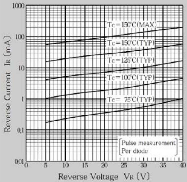
Reverse Current
