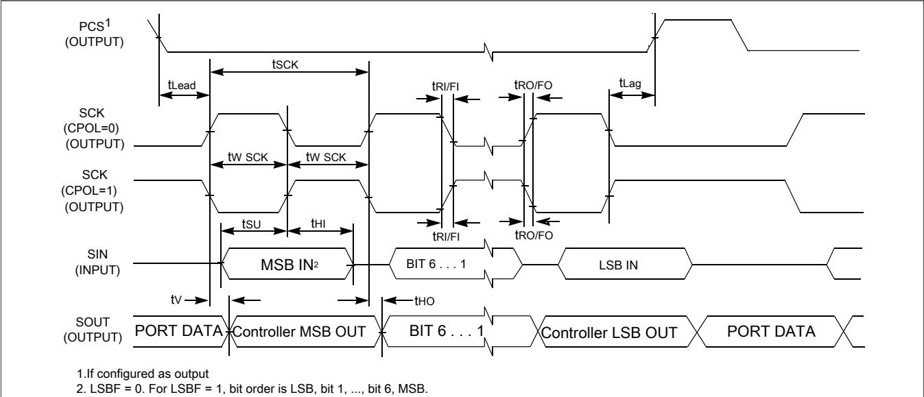
Figure 35. LPSPI Controller mode timing (CPHA = 1)
