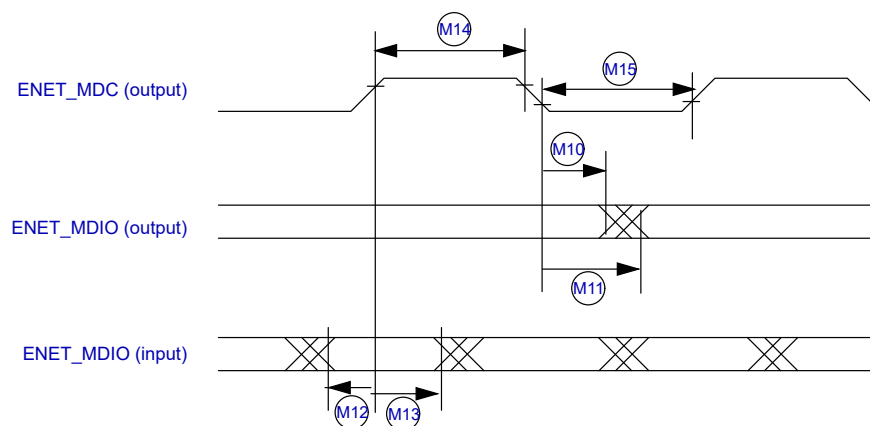
Figure 27. MII serial management channel timing diagram
