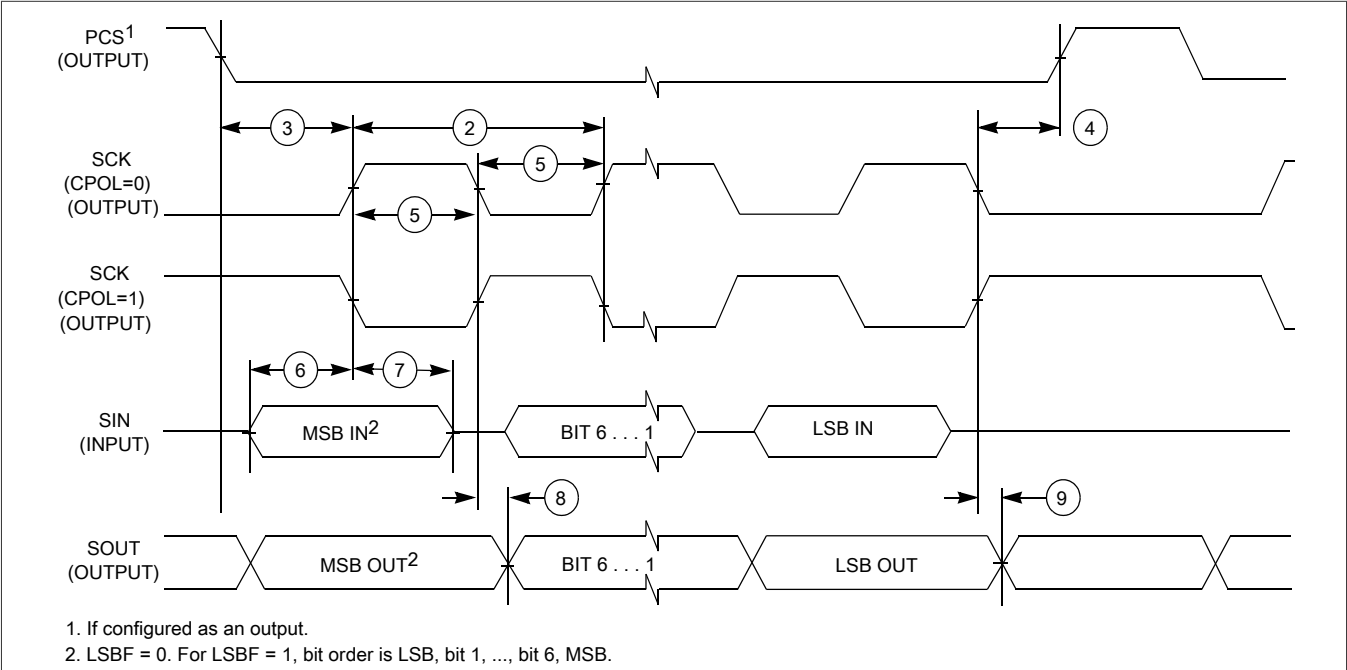
Figure 34. LPSPI Controller mode timing (CPHA = 0)
