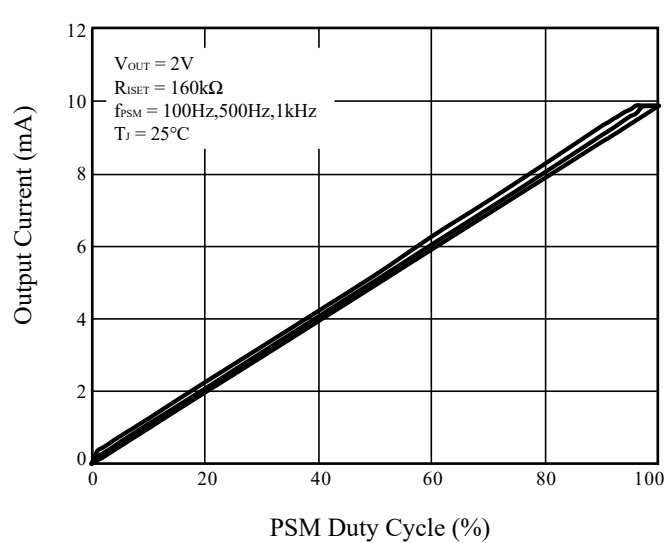
Figure 19 Output Current vs. PSM Duty Cycle
