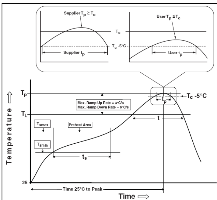
Figure 47 Classification Profile
