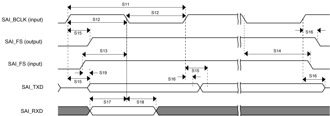
Figure 15. SAI Timing — Target Mode
