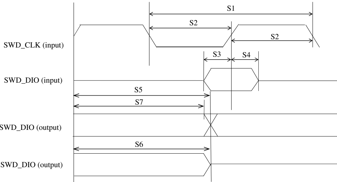
Figure 12. SWD timing
