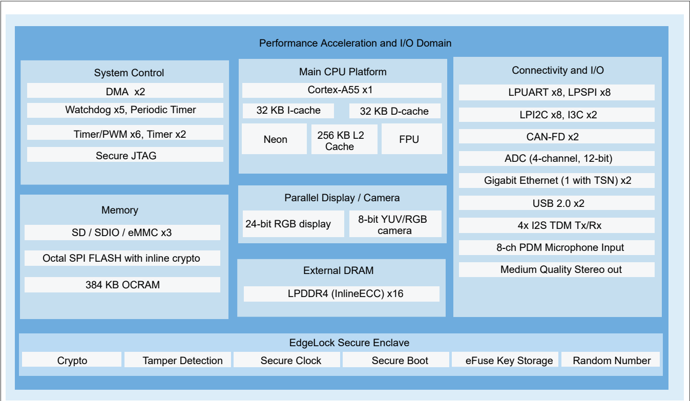
Figure 2. i.MX 91 system block diagram
