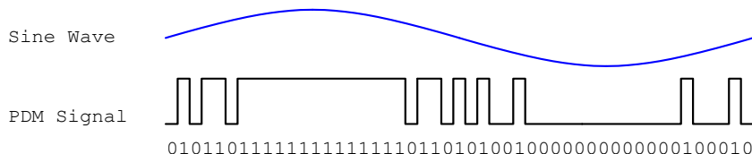
Figure 25. PDM representation of a sine wave
