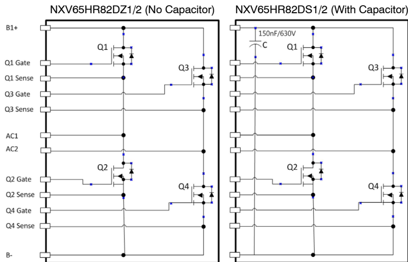
Figure 2. Schematic
