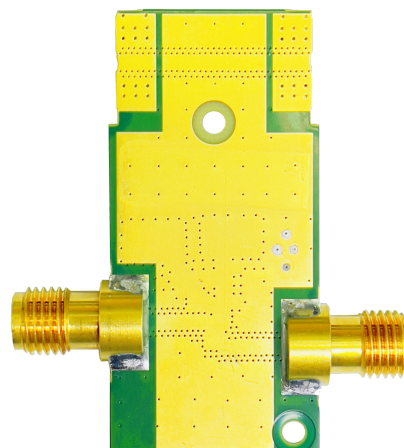
Figure 2. ADL8105-EVALZ Secondary Side
