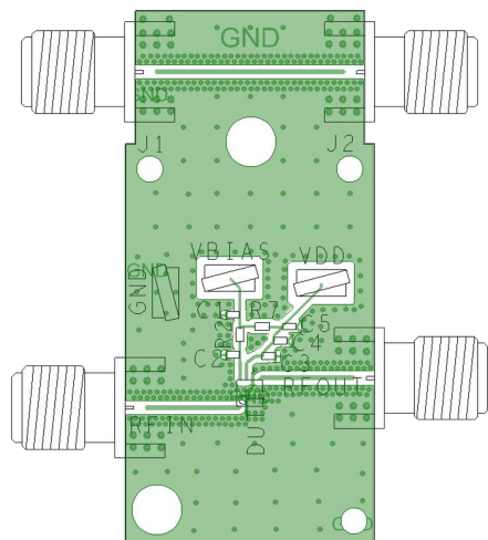
Figure 5. ADL8105-EVALZ Assembly Drawing (J1 and J2 Are Not Installed)
