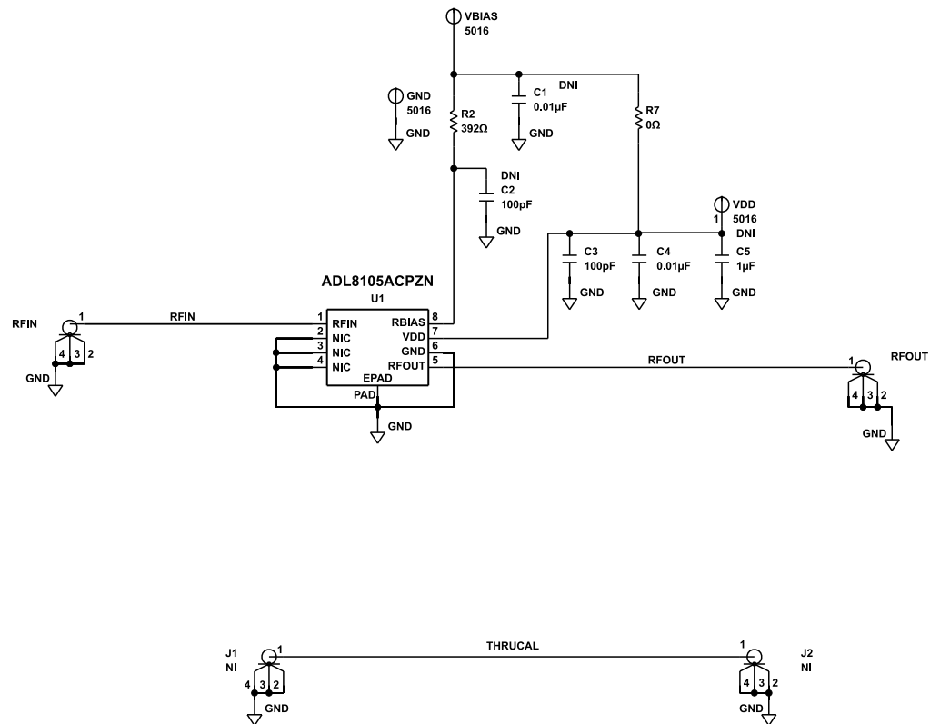
Figure 4. ADL8105-EVALZ Schematic
