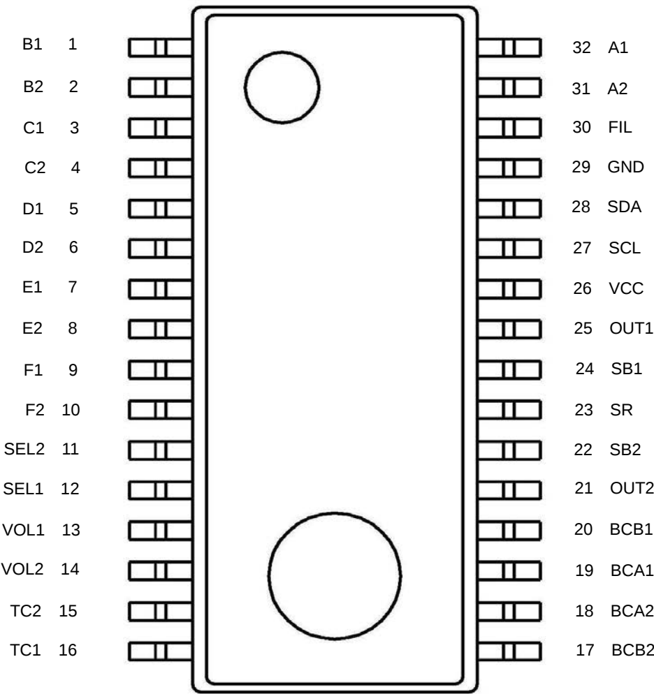
Figure 2. Pin Configuration
