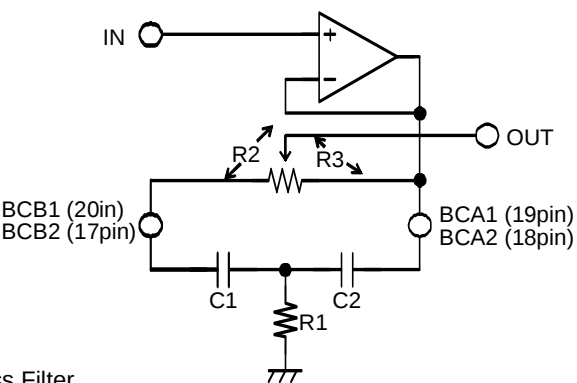
Figure 18. Bass Filter
