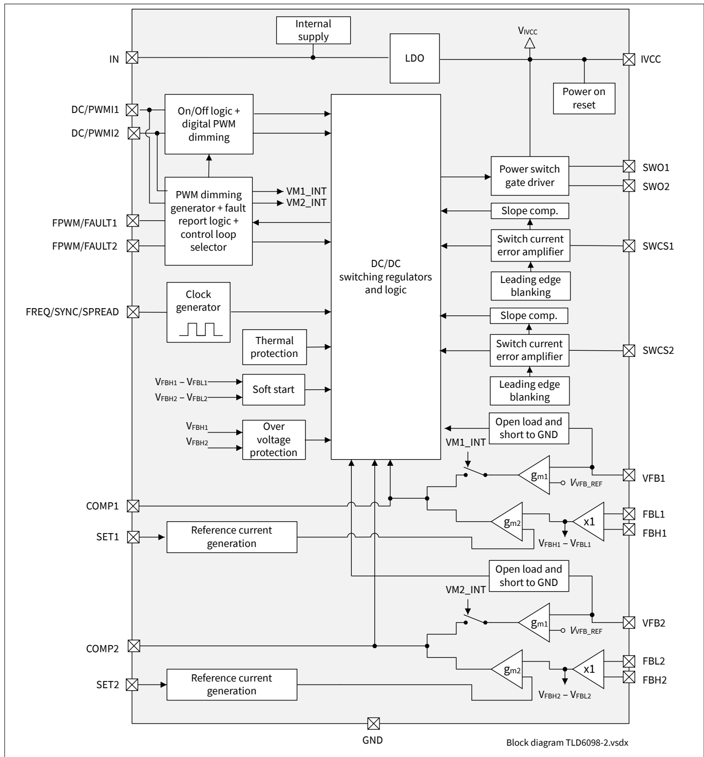
Figure 2 Block diagram
