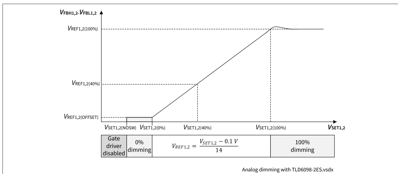
Figure 13 Relationship between V_{SET1,2} and the respective voltage V_{REF1,2}
