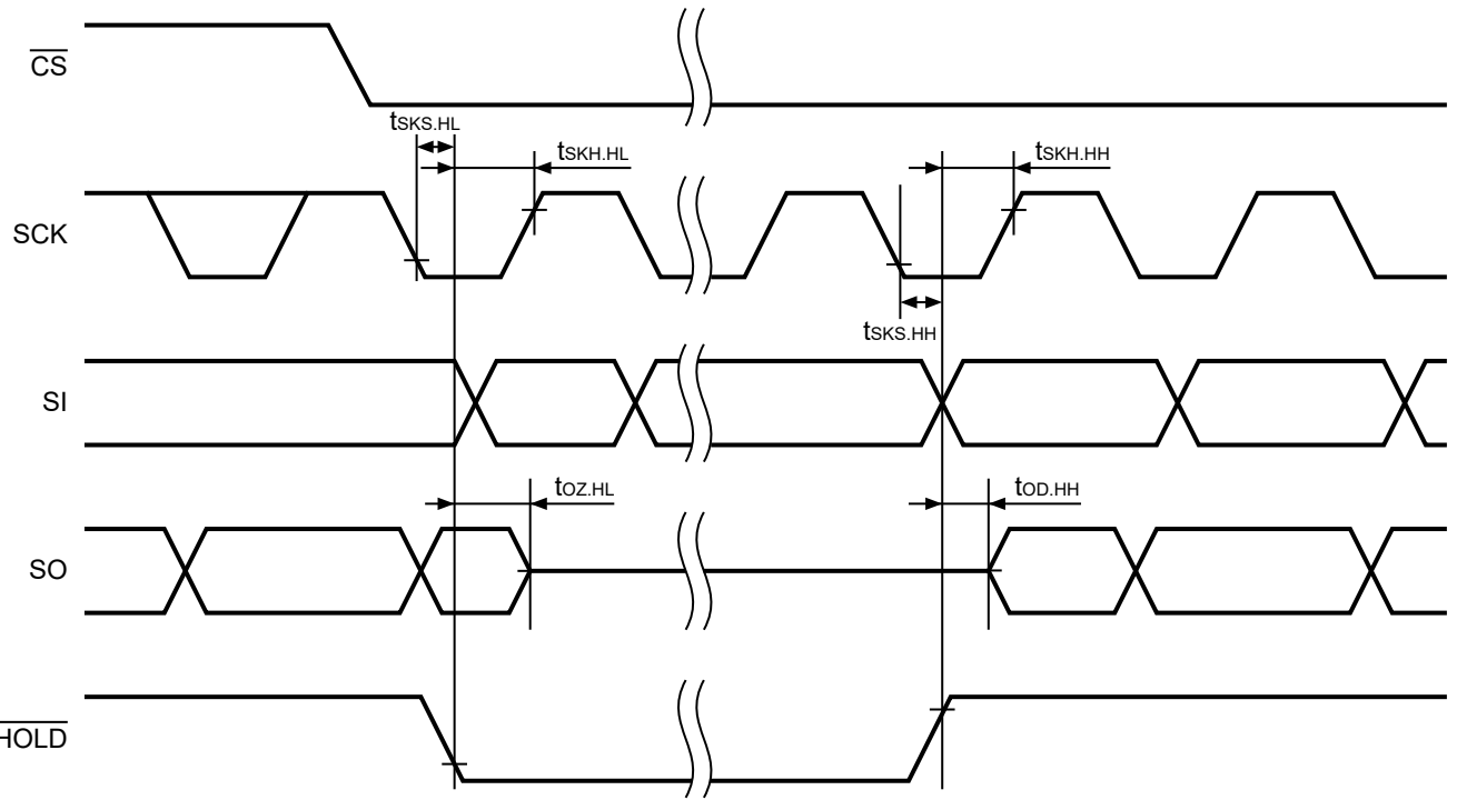
Figure 7 Hold Timing
