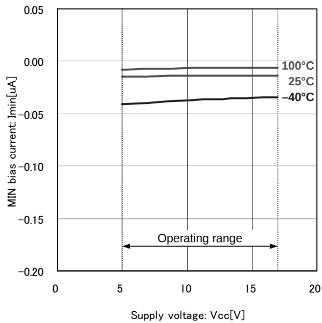
Fig.24 MIN bias current
