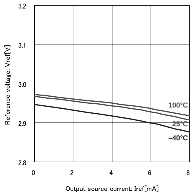
Fig.21 Reference voltage current ability (Vcc=12V)
