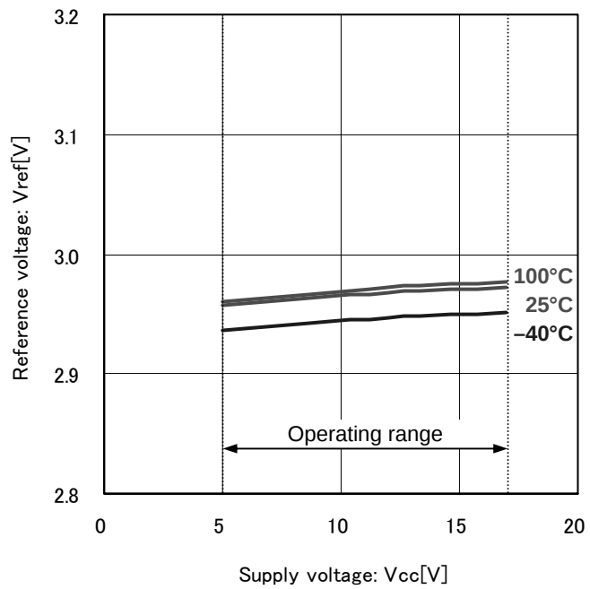
Fig.20 Reference voltage
