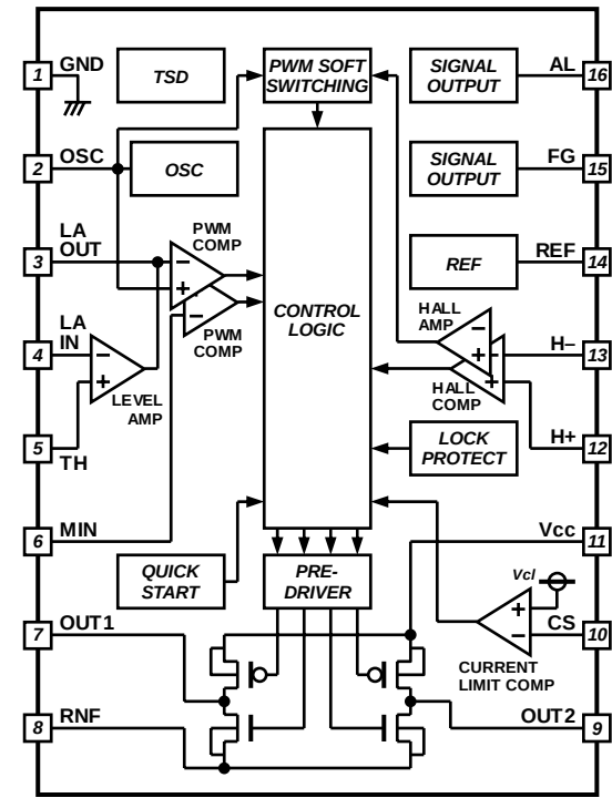
Fig.2 Block diagram
