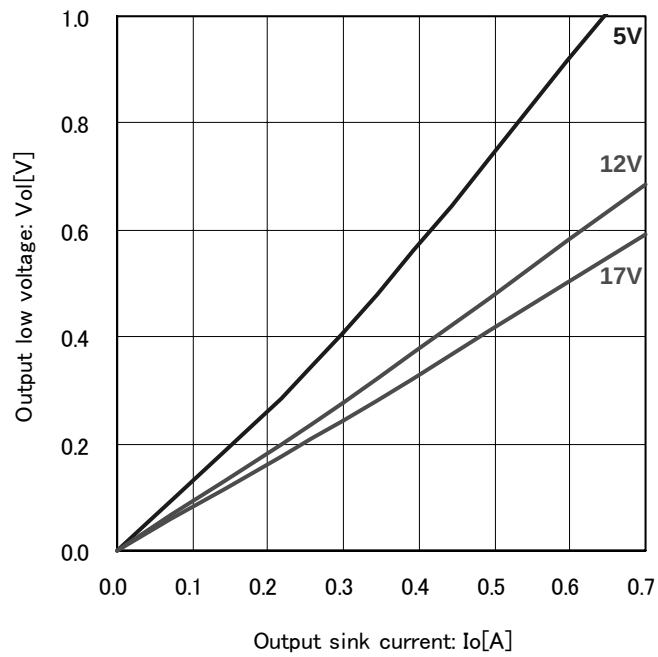
Fig.8 Output low voltage ( T_a=25^\circ C )
