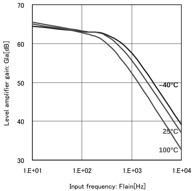
Fig.16 Level amplifier gain (V cc =12V)
