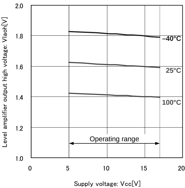
Fig.18 Level amplifier output high voltage
