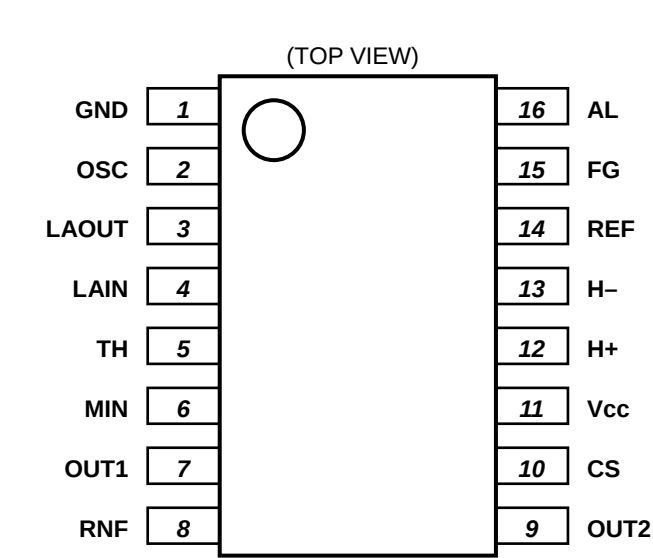
Fig.1 Pin configuration
