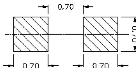
Figure 1. IN-S63BT Solder Pattern
