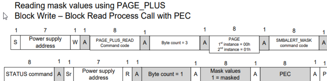
Figure 8. PAGE_PLUS_READ command.
