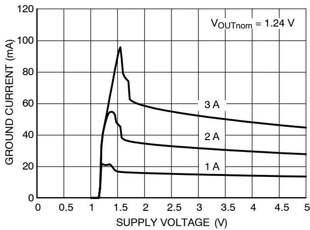
Figure 10. Ground Current vs. Supply Voltage
