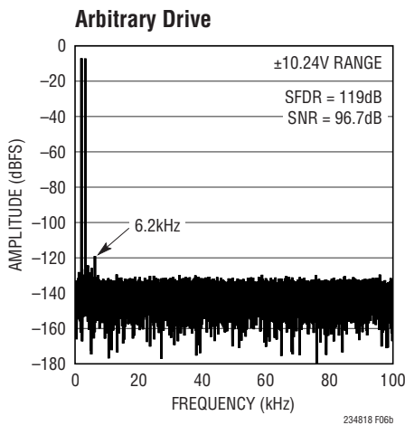
Figure 6b. Two-Tone Test. IN^+ = -7\text{dBFS} 2kHz Sine, IN^- = -7\text{dBFS} 3.1kHz Sine, 32k Point FFT, f_{\text{SMP}_L} = 200\text{ksps} . Circuit Shown in Figure 6a with LT1469 Amplifiers, R_{\text{FILT}} = 49.9\Omega , C_{\text{FILT}} = 1000\text{pF}
