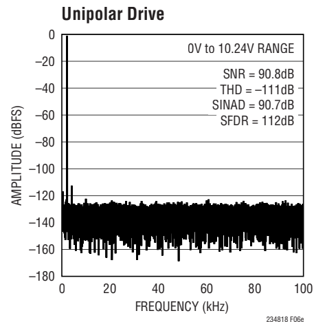
Figure 6e. IN^+ = -1\text{dBFS} 2kHz Unipolar Sine, IN^- = 0\text{V} , 32k Point FFT, f_{\text{SMP}_L} = 200\text{ksps} . Circuit Shown in Figure 6a with LT1469 Amplifiers, R_{\text{FILT}} = 49.9\Omega , C_{\text{FILT}} = 1000\text{pF}
