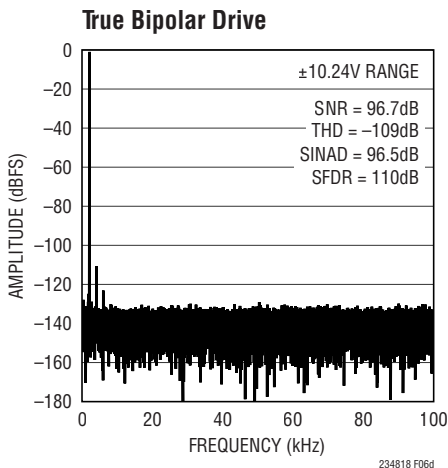
Figure 6d. IN^+ = -1\text{dBFS} 2kHz True Bipolar Sine, IN^- = 0\text{V} , 32k Point FFT, f_{\text{SMP}_L} = 200\text{ksps} . Circuit Shown in Figure 6a with LT1469 Amplifiers, R_{\text{FILT}} = 49.9\Omega , C_{\text{FILT}} = 1000\text{pF}
