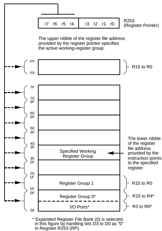
Figure 18. Register Pointer
