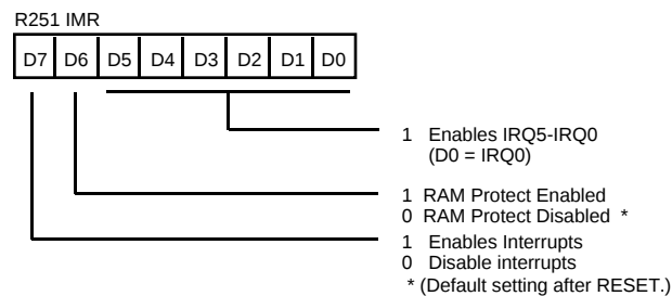
Figure 62. Interrupt Mask Register (FB H : Read/Write)
