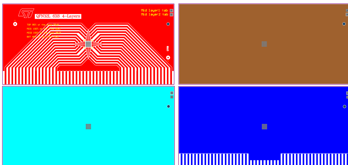
Figure 47. QFN 6x6 PCB 4 layers
