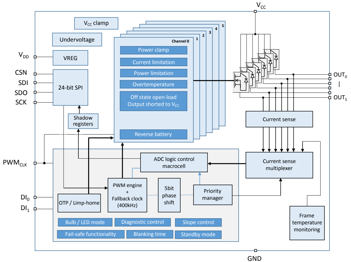
Figure 1. Block diagram
