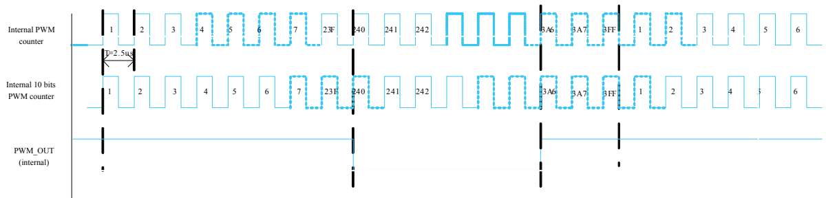
Figure 15. Resulting waveform 4
