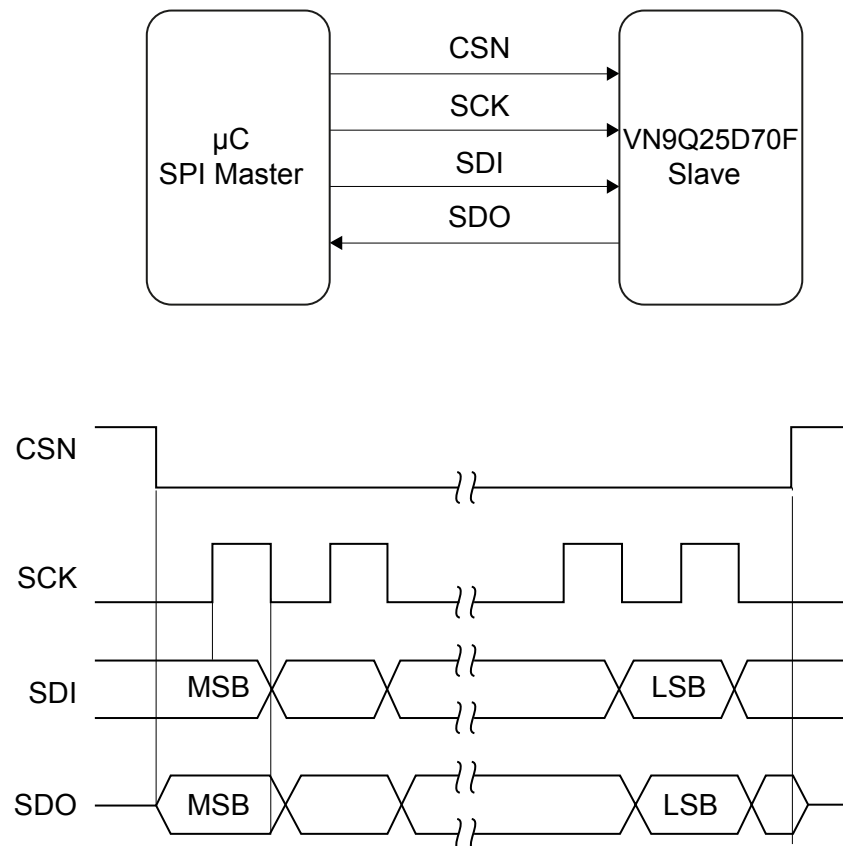
Figure 6. Supported SPI mode
