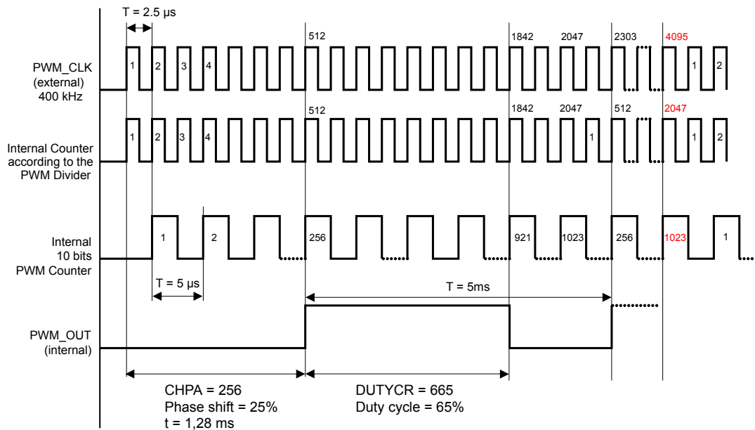
Figure 12. Resulting waveform 1
