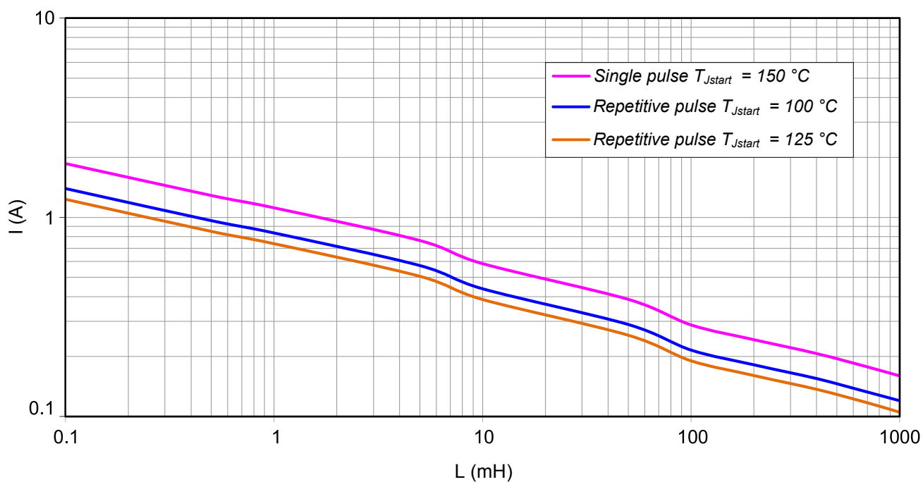
Figure 39. Maximum turn off current versus inductance Ch0,5 – LED mode
