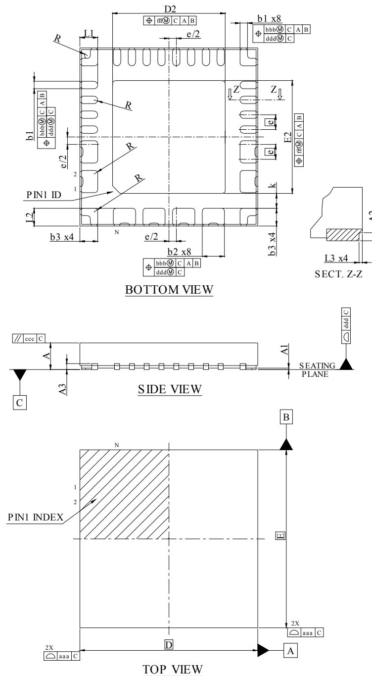
Figure 52. QFN 6x6 package outline
