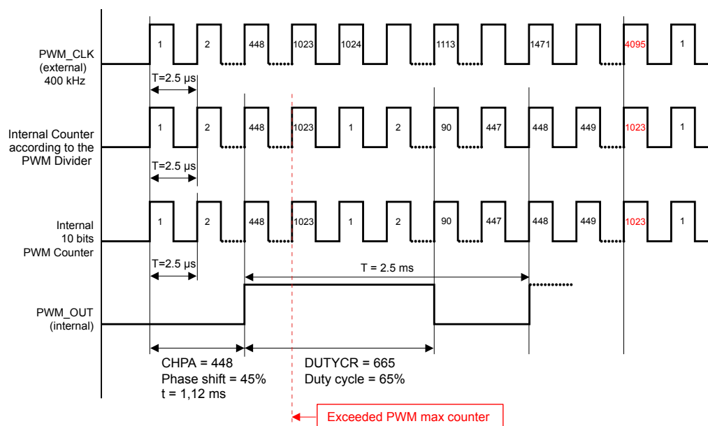
Figure 13. Resulting waveform 2
