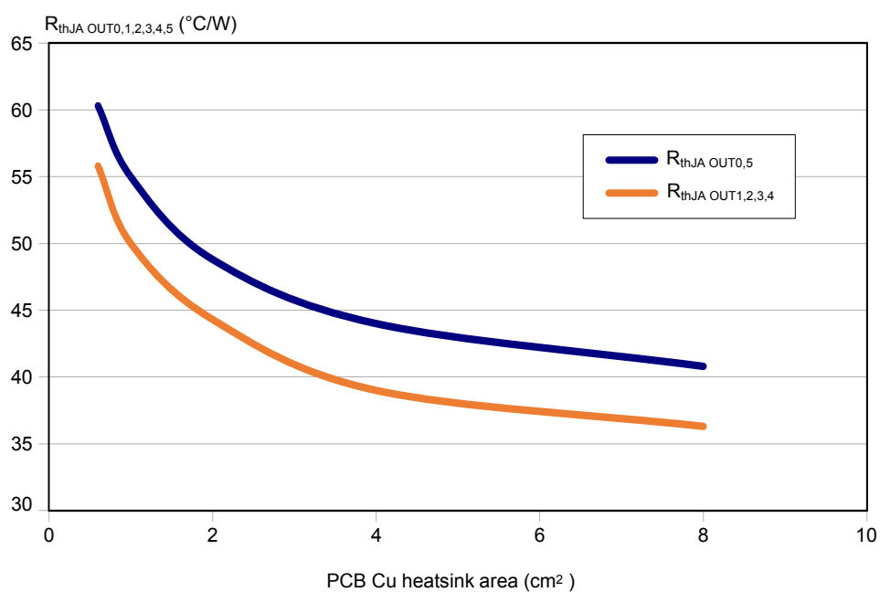
Figure 48. R_{thJA} vs PCB copper area in open box free air conditions
