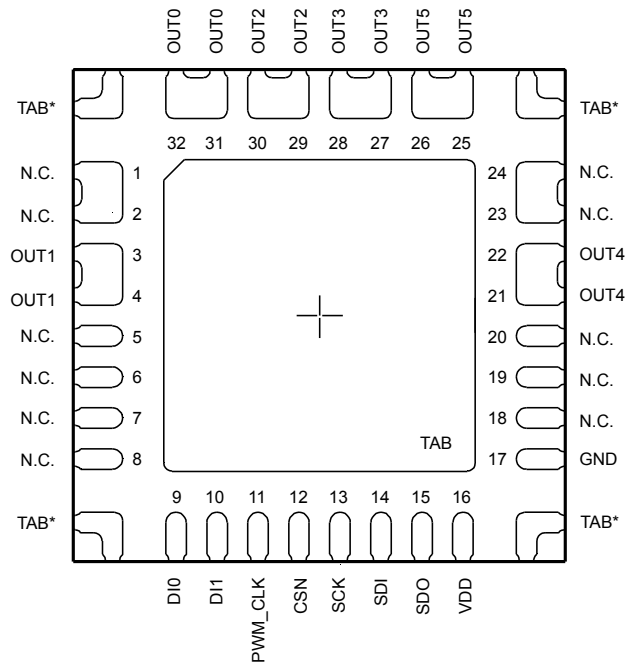
Figure 2. Connection diagram (top view)
