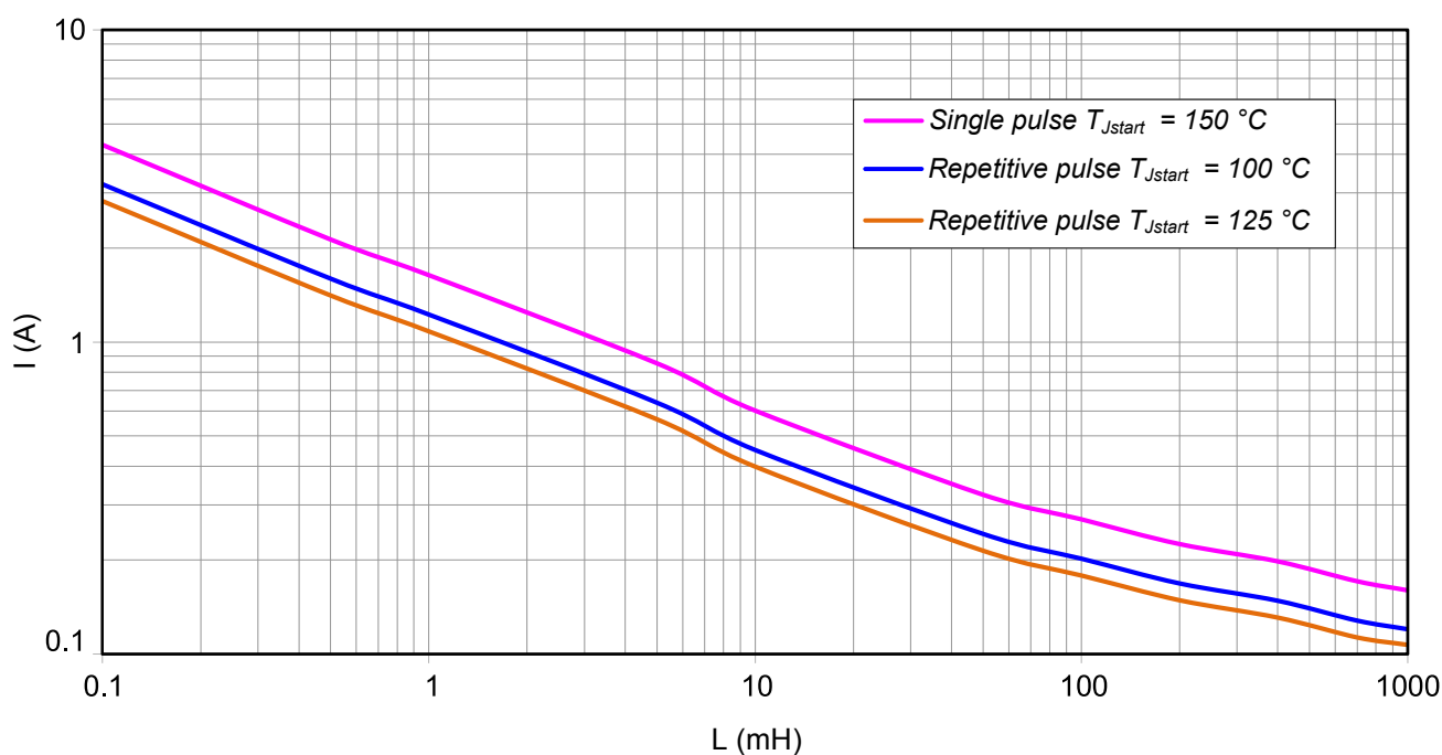
Figure 37. Maximum turn off current versus inductance Ch0,5 – Bulb mode
