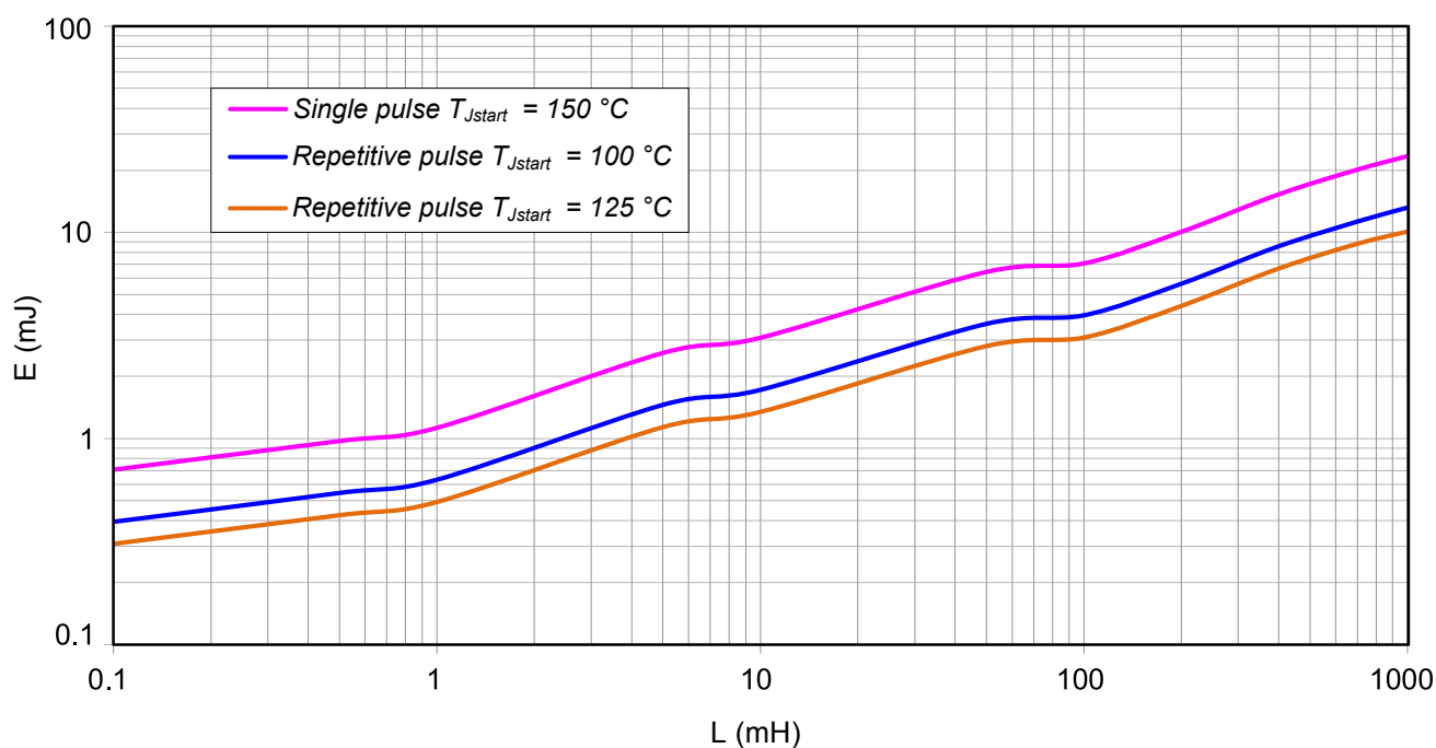
Figure 43. Maximum turn off energy versus inductance Ch0,5 – LED mode
