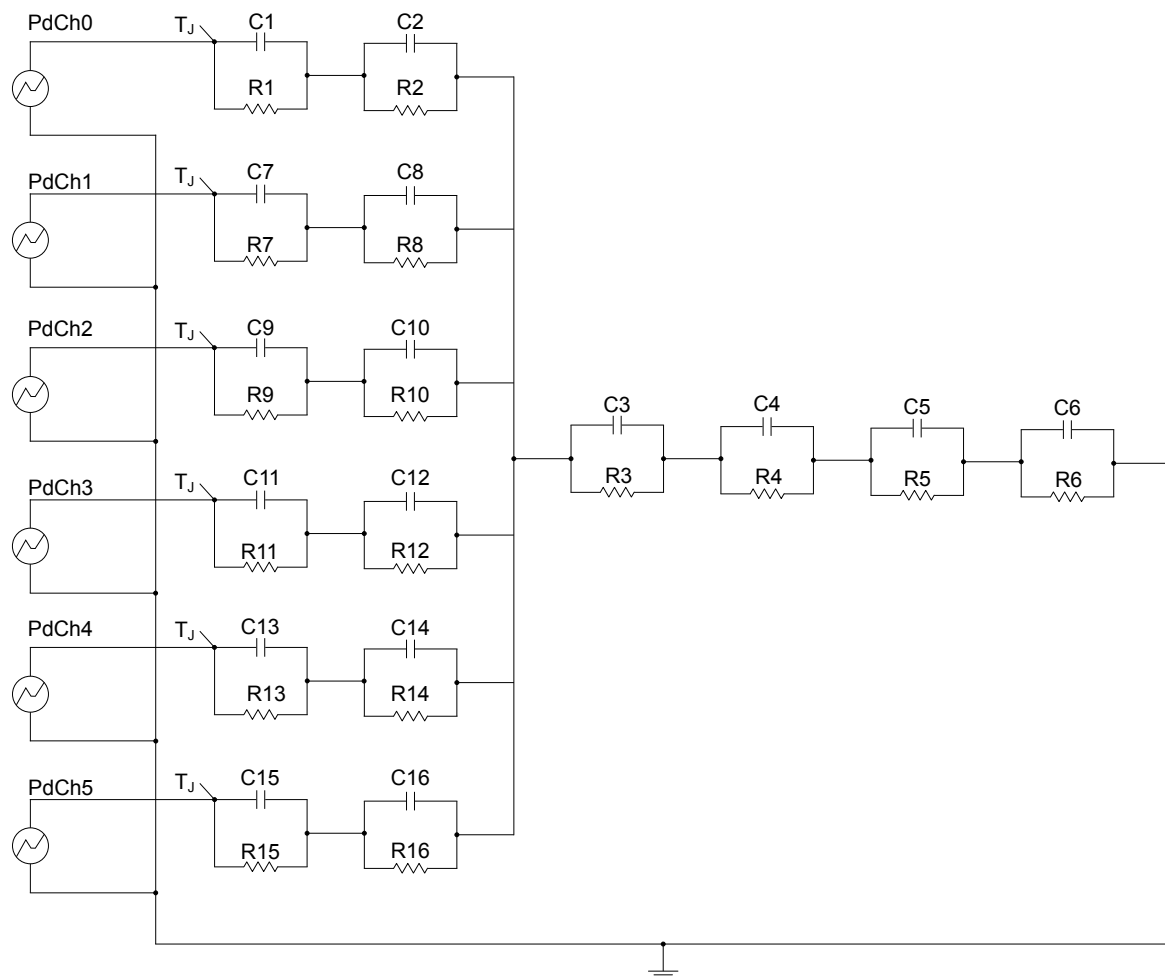
Figure 51. Thermal fitting model
