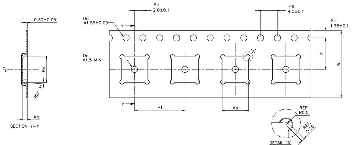
Figure 54. QFN 6x6 carrier tape
