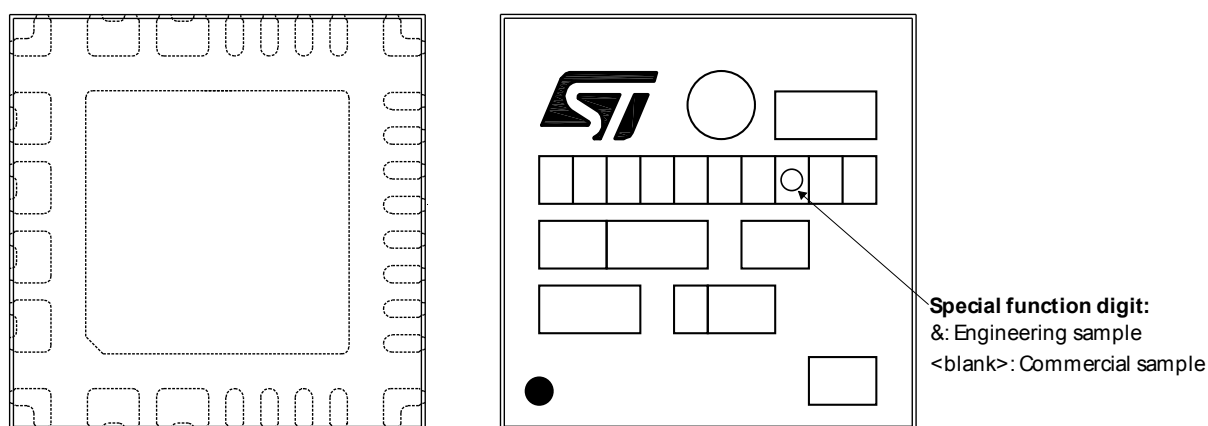
Figure 55. QFN 6x6 marking information
