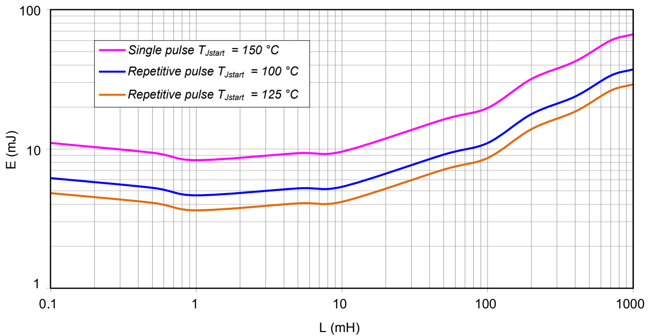
Figure 40. Maximum turn off energy versus inductance Ch1,2,3,4 – Bulb mode
