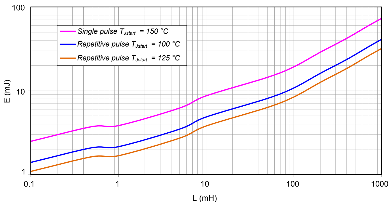
Figure 42. Maximum turn off energy versus inductance Ch1,2,3,4 – LED mode
