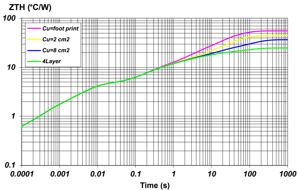
Figure 50. QFN 6x6 thermal impedance junction ambient for channels 1,2,3,4
