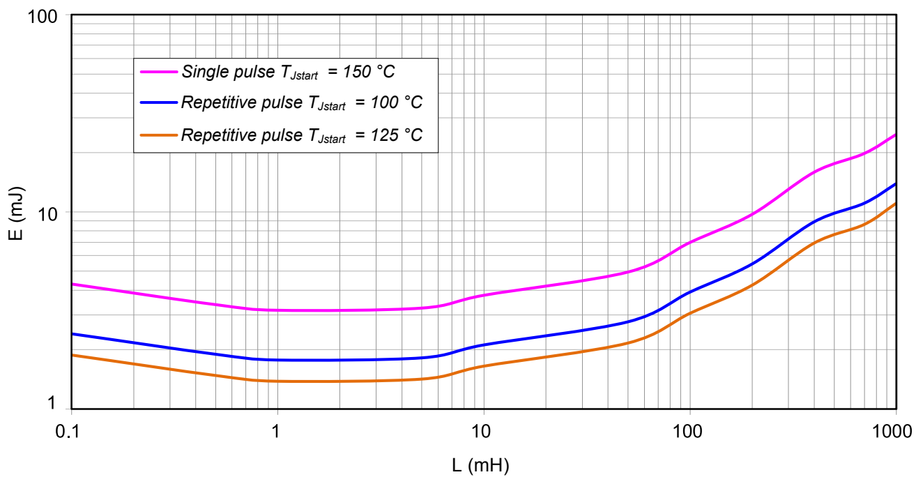
Figure 41. Maximum turn off energy versus inductance Ch0,5 – Bulb mode
