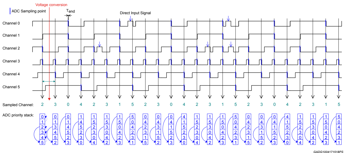
Figure 21. Sequence of channels
