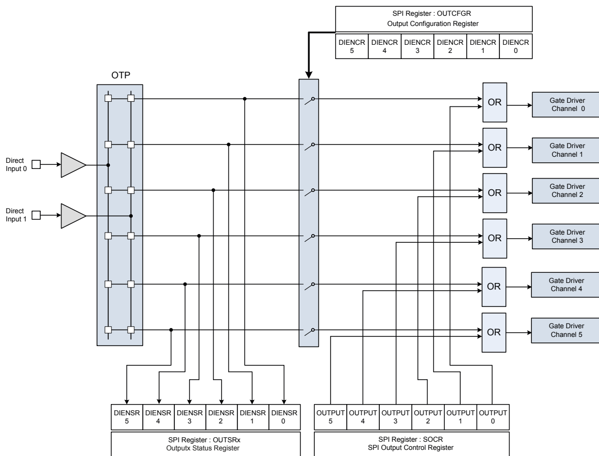
Figure 16. 6-channel direct input block diagram
