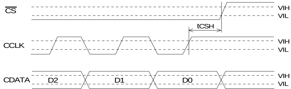
Control Data Interface Timing2
