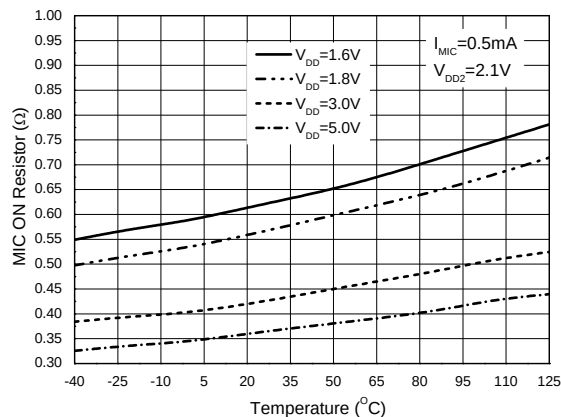
MIC ON Resistor vs. Temperature
