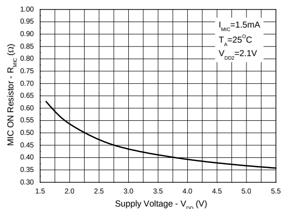
MIC ON Resistor vs. Supply Voltage
