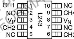
10-Lead MSOP-10
